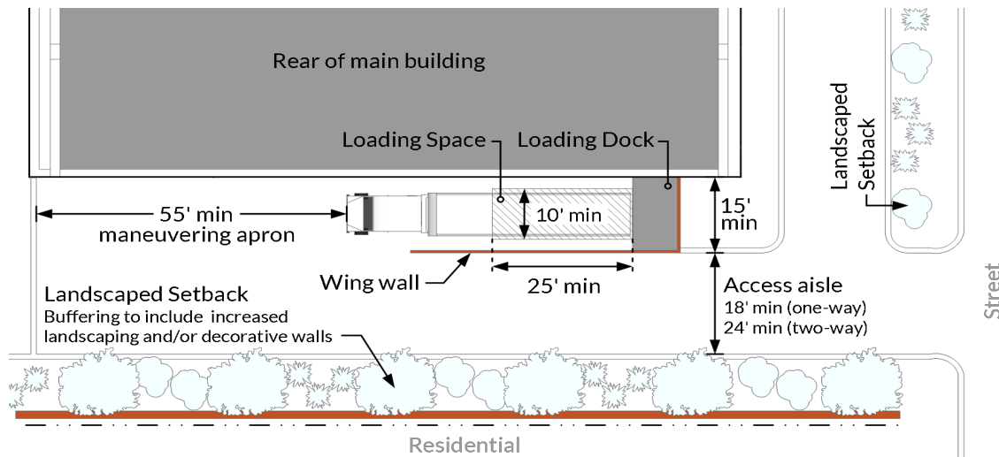
Figure 30.04-18: Loading Area Design
