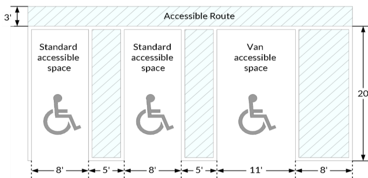
Figure 30.04-4: Accessible Space and Access Design
