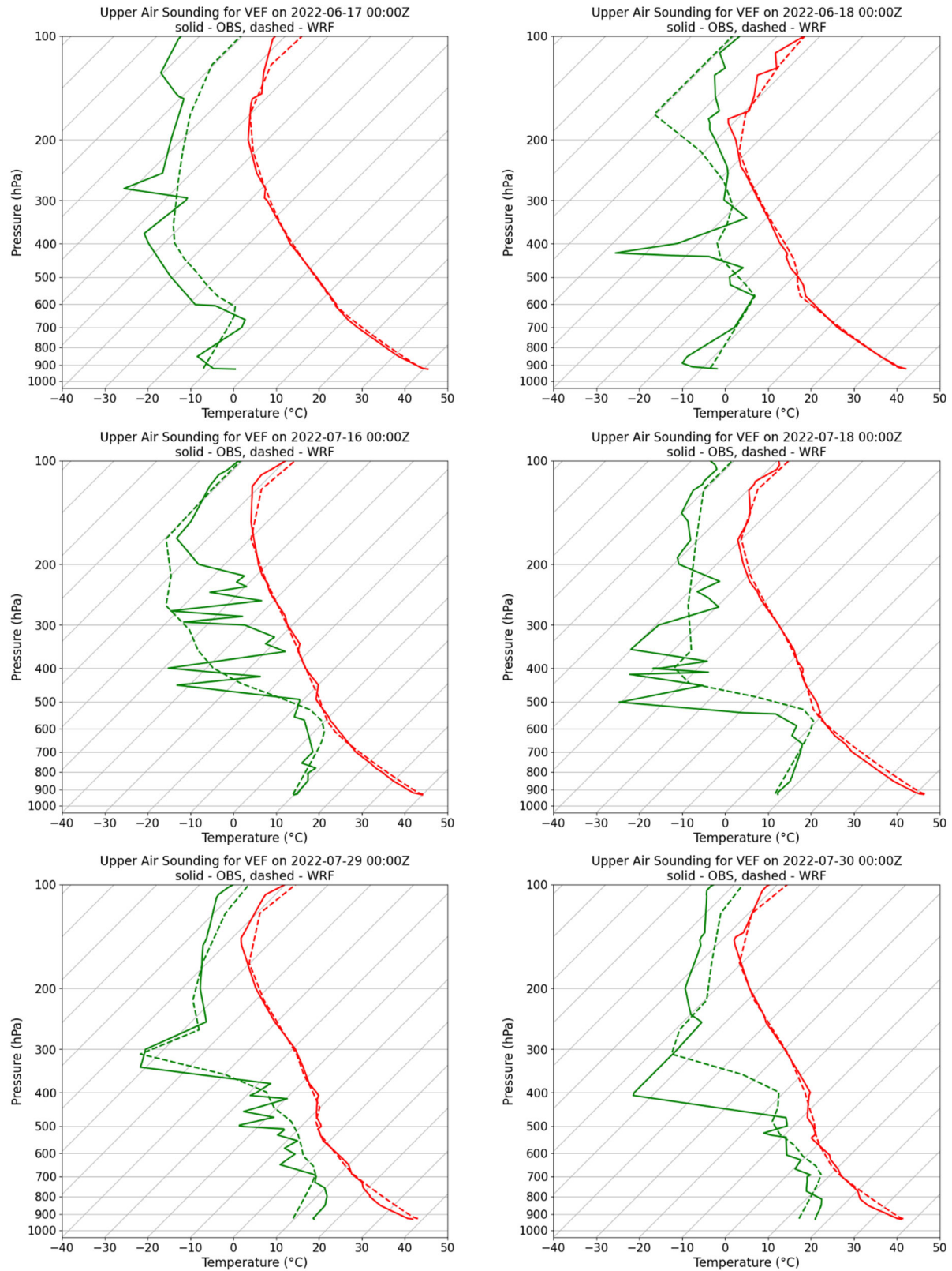
Figure 5-9. Vertical profiles of observed (solid) and WRF (dashed) temperature (red) and dewpoint temperature (green) at 5 PM PDT (00 UTC) on ozone exceedance days in 2022.
