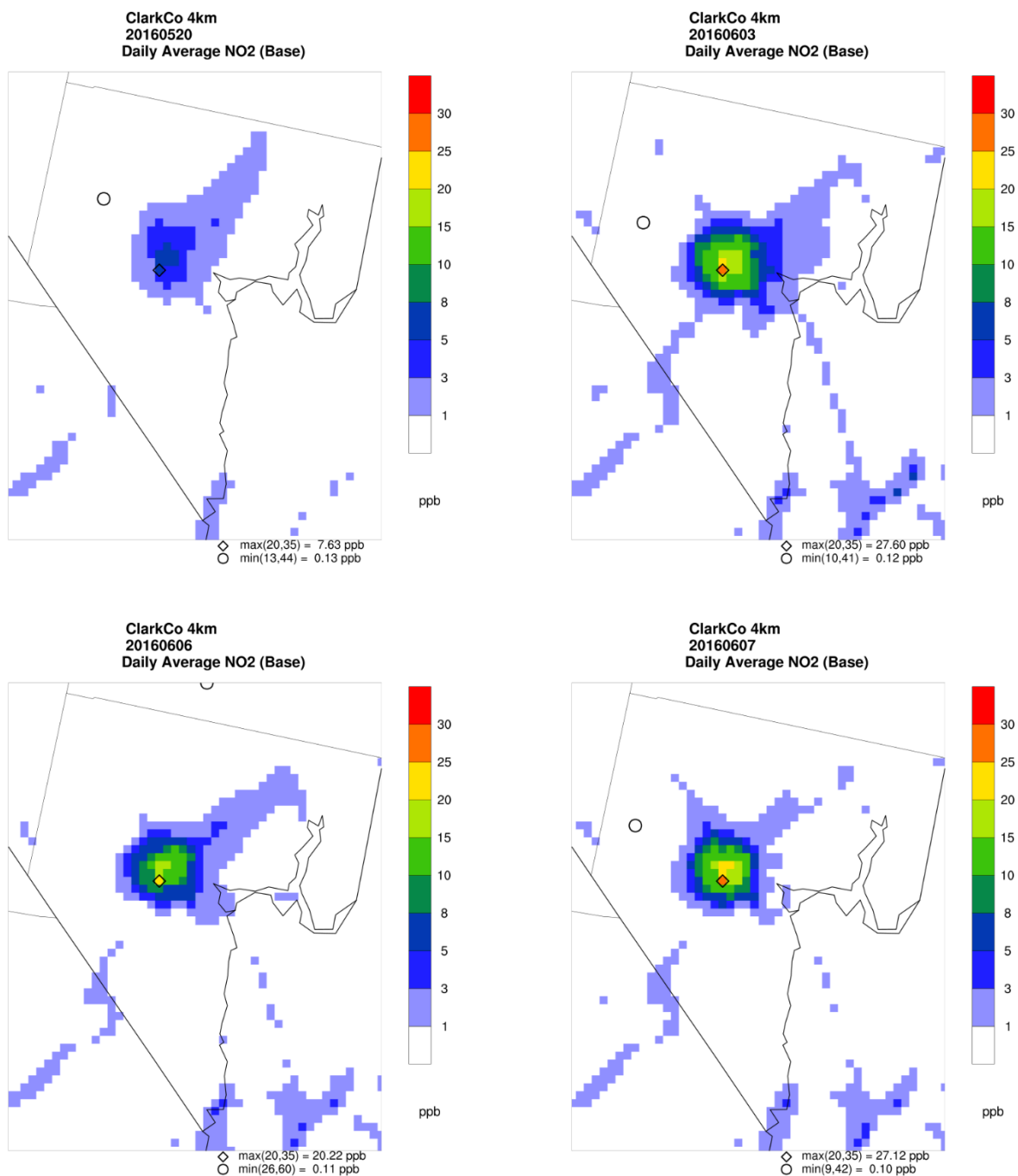
Figure 8-5. Spatial plots of predicted 24-hr daily average NO 2 modeled concentrations on 26 high ozone dates in 2016 when at least one peak measurement exceeded 70 ppb.
