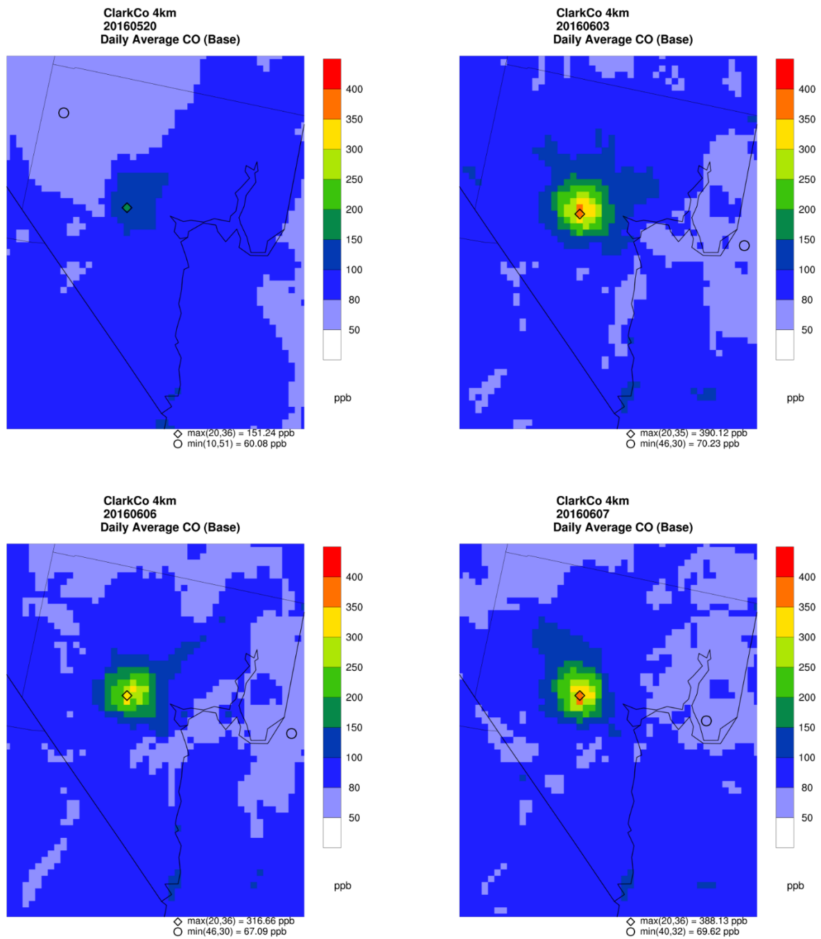
Figure 8-6. Spatial plots of predicted 24-hr daily average CO modeled concentrations on 26 high ozone dates in 2016 when at least one peak measurement exceeded 70 ppb.
