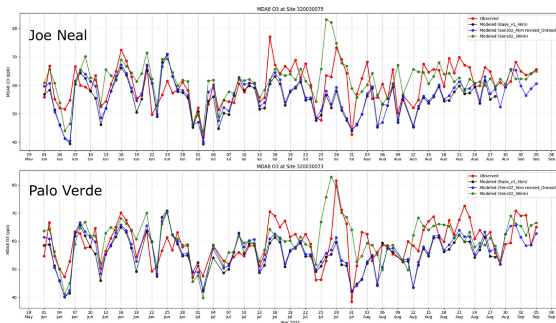
Figure 8-2. Time series of MDA8 ozone over the entire 2022 modeling period at the Joe Neal (top) and Palo Verde (bottom) monitoring sites. Daily AQ5 measurements are shown in red, the Base_v1 case is shown in black, the Sens02_rev case with corrected on-road VOC emissions is shown in blue, and the Sens02 case from the 36US3 run is shown in green.
