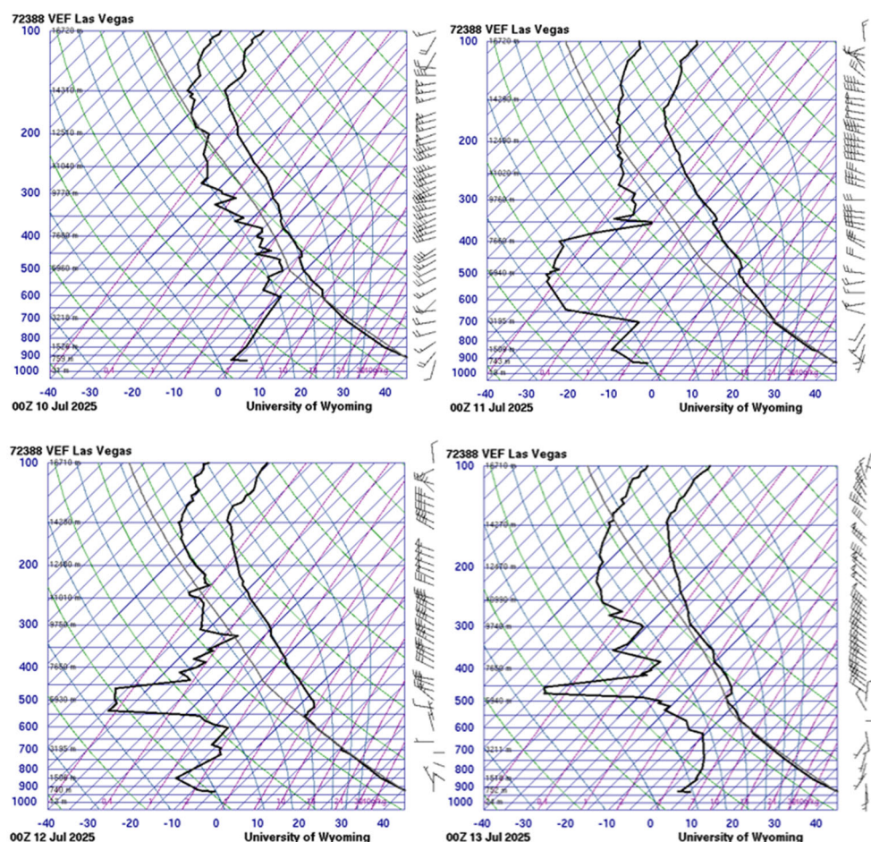
Figure 280. Observed soundings at 16:00 PST on July 9 (top left), July 10, (top right), July 11 (bottom left), and July 12 (bottom right). Images courtesy of the University of Wyoming.
