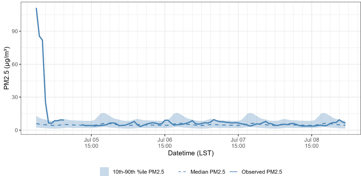
PM2.5 - Joe Neal (320030075) 2023-07-05 to 2023-07-08
