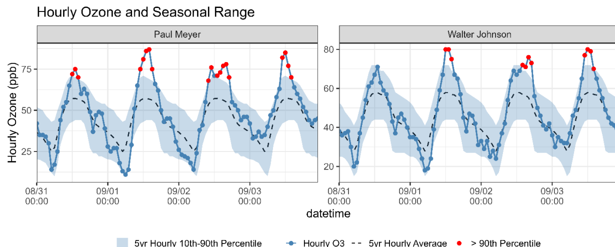
Figure 180. Hourly ozone concentrations (ppb) recorded at the Paul Meyer site across August 31-September 4, 2022, compared to 5-yr ozone season (May 1-October 31) hourly means and 10-90th percentiles.
