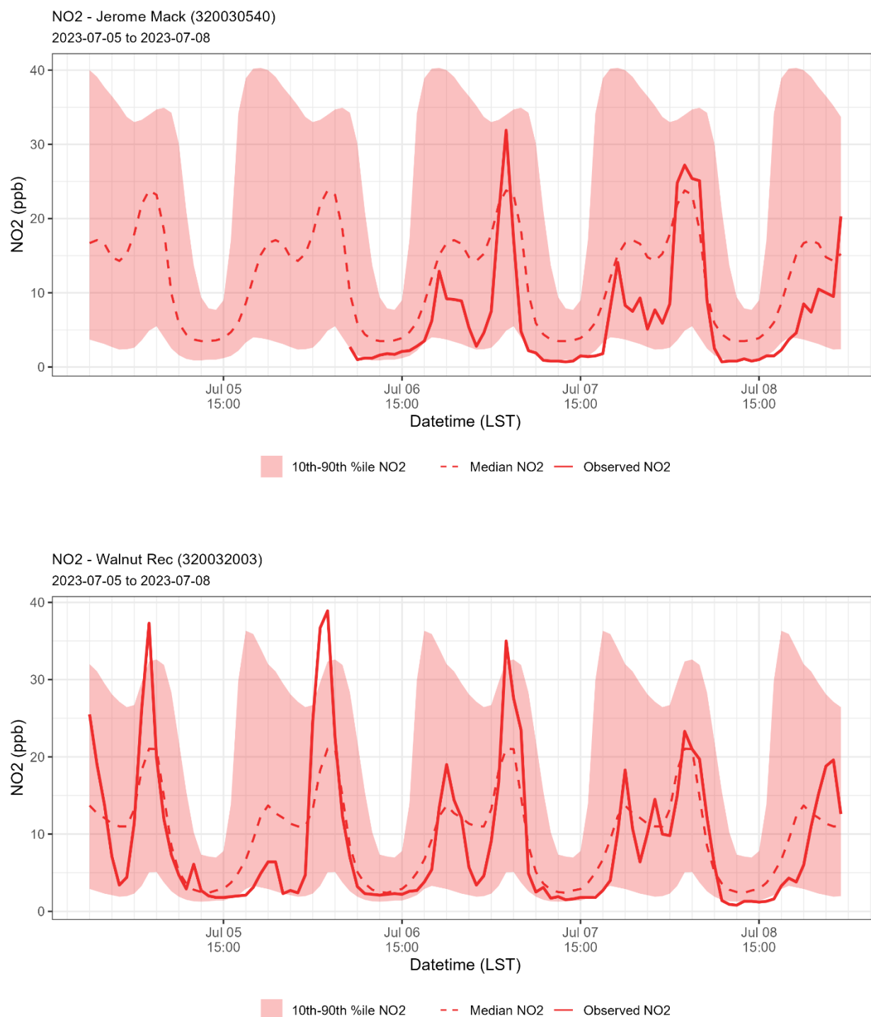
Figure 240. Hourly NO 2 measurements overlaid on the 10th to 90th percentile diurnal concentration at Joe Neal (AQS site code 320030075), Jerome Mack (AQS site code 320030540), and Walnut Recreation (AQS site code 320032003). The 10th to 90th percentile concentration is calculated across the ozone production season (April-September) for 2018-2023. Note: Walnut Recreation only includes data from June 1, 2021 and onwards.
