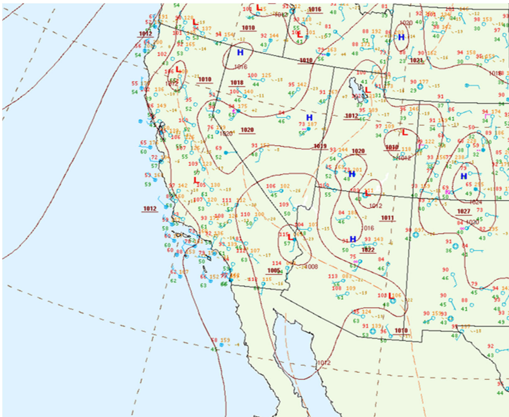
Figure 324. Surface weather conditions at 16:00 PST on July 24, 2024. Surface pressure (mb) indicated by dark red contours and underlined numbers. High and low pressures identified by blue "H" and red "L", respectively. Source: NOAA Weather Prediction Center.
