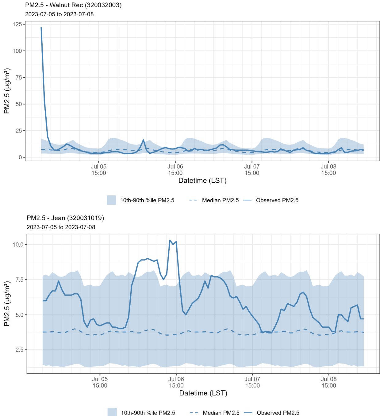
Figure 242. Hourly PM 2.5 measurements overlaid on the 10th to 90th percentile diurnal concentration at Jerome Mack (AQ5 site code 320030540), Liberty (AQ5 site code 320030299), Green Valley (AQ5 site code 320030298), Joe Neal (AQ5 site code 320030075), Palo Verde (AQ5 site code 320030073), Walter Johnson (AQ5 site code 320030071), Mountain's Edge (AQ5 site code 320030044), Paul Meyer (AQ5 site code 320030043), Walnut Recreation (AQ5 site code 320032003), and Jean (AQ5 site code 320031019). The 10th to 90th percentile concentration is calculated across the ozone production season April-September for 2018-2023. Note: Walnut Recreation includes data from June 1, 2021, and onwards; Mountain's Edge includes data from October 1, 2020, and onwards; Liberty includes data from May 1, 2021, and onwards.
