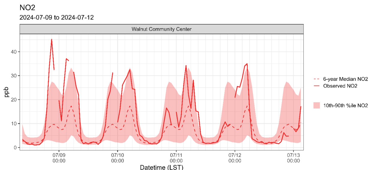
Figure 294. Hourly NO 2 concentrations for July 9-13 overlaid on the 10th-to-90th percentile diurnal concentration at Walnut Community Center* (AQS site code 320032003). The 10th-to-90th percentile concentration is calculated across the ozone production season (April-September) of 2021-2024. Note: the Walnut Community Center site only includes data from June 1, 2021, and onwards.
