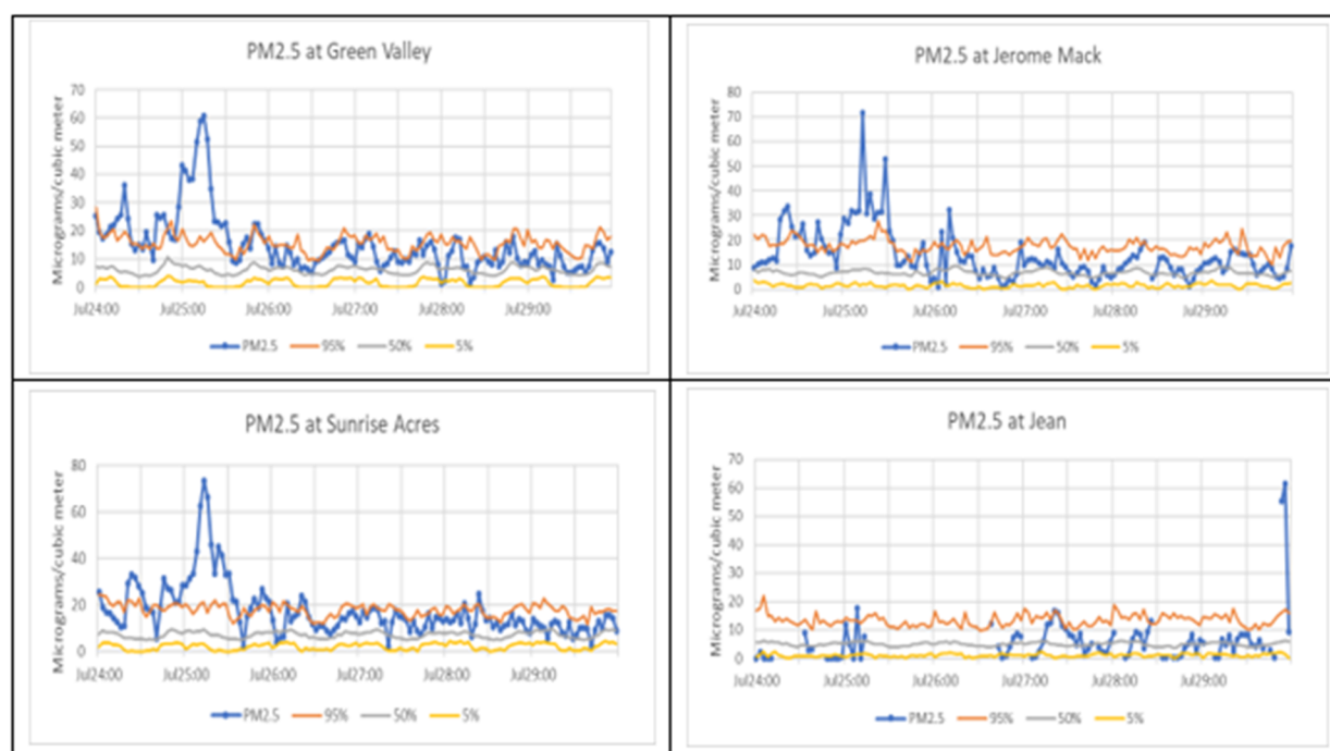
Figure 24. 6-yr hourly seasonal 95th, 50th, and 5th percentiles for PM 2.5 concentrations (µg/m 3 ) at LVV FEM monitors during July 24-29, 2016.
