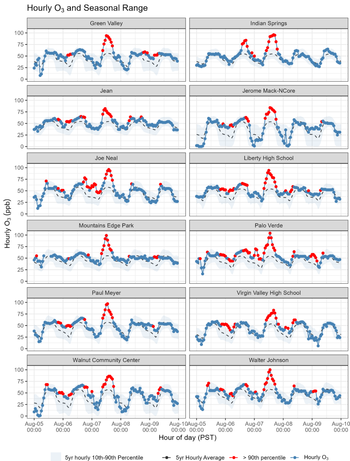
Figure 91. Hourly ozone concentrations (ppb) compared to 5-yr* ozone season (May 1-October 31) hourly means and 10-90th percentiles. *Note: data collection began in 2020 at the Mountain's Edge site, and in 2021 at the Liberty High School, Virgin Valley High School, and Walnut Community Center sites.
