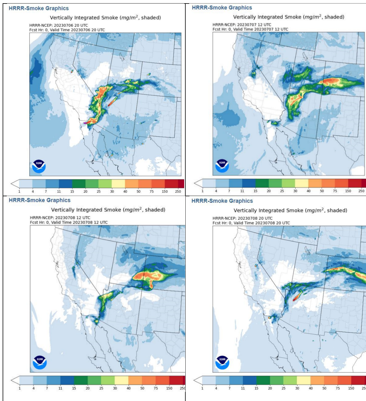
Figure 218. HRRR vertically integrated smoke forecast for July 5-8, 2023, at 05:00 and 13:00 PST.
