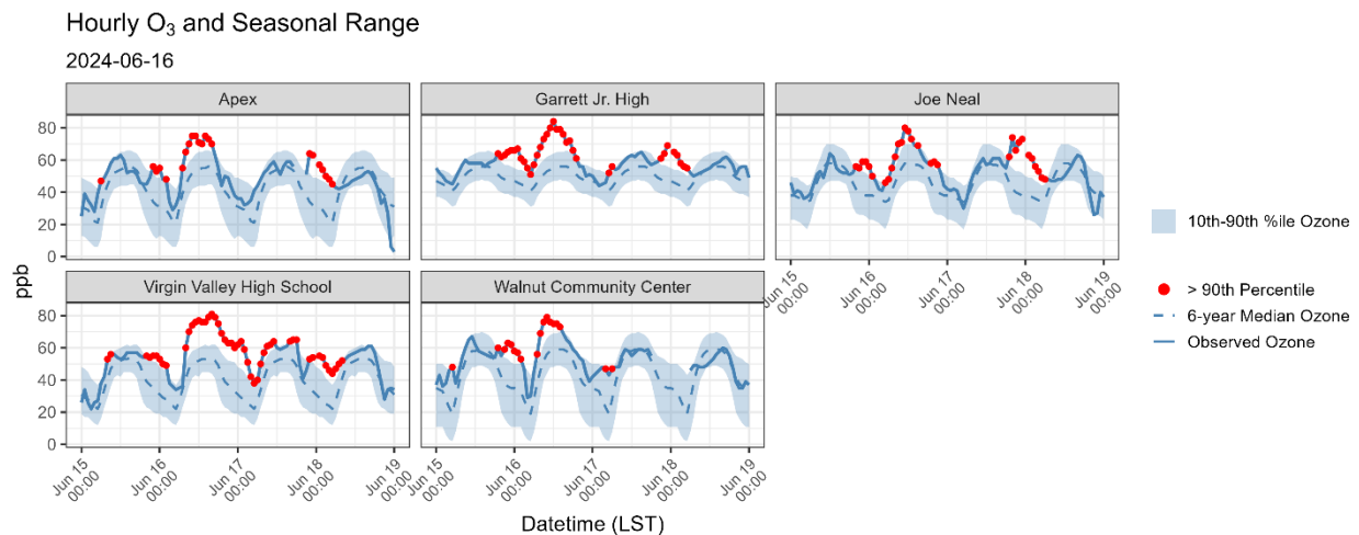
Figure 249. Hourly ozone concentrations (ppb) compared to 6-year ozone season (April 1 – September 30) hourly medians and 10th-to-90th percentiles. Red points indicate hourly ozone concentrations that exceeded the 90th percentile. Note: the Apex site only includes data from June 1, 2023, and onwards; the Garrett Jr. High site only includes data from April 1, 2021, and onwards; the Virgin Valley High School only includes data from 2021, and onwards; and the Walnut Community Center site only includes data from June 1, 2021, and onwards.
