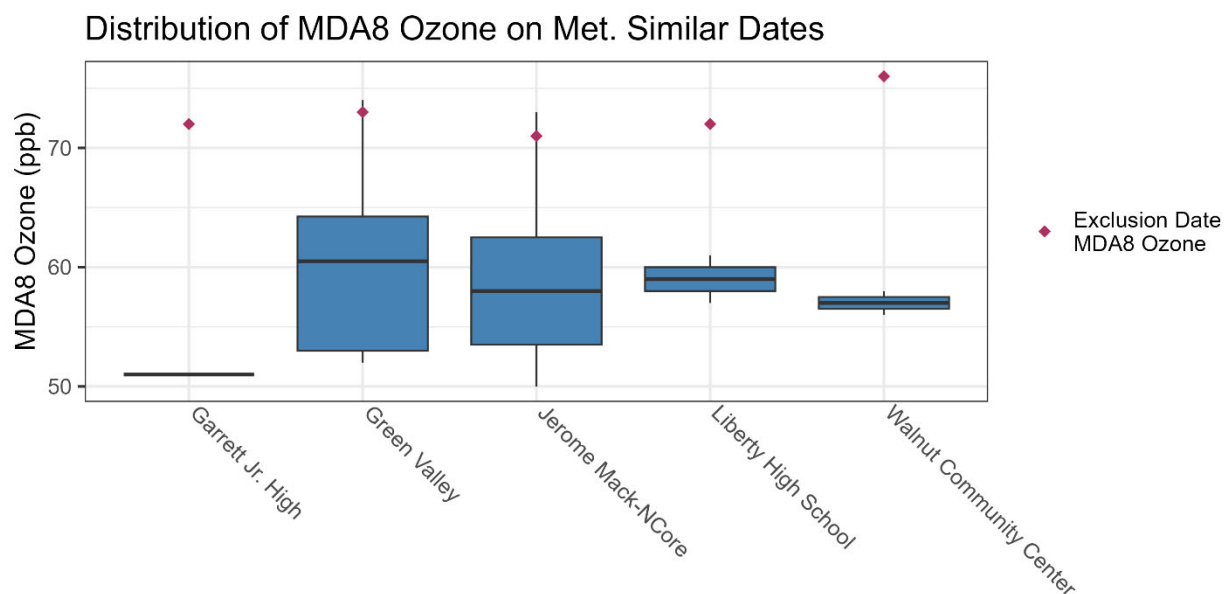
Figure 162. Distribution of MDA8 ozone concentrations on meteorologically similar days at measurement sites that were in exceedance on the exclusion date (blue boxes). MDA8 ozone concentrations measured on the exclusion date (July 17, 2022) at each site are plotted as red diamonds.
