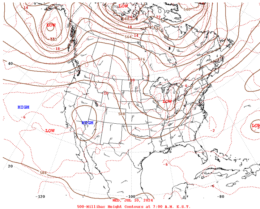
Figure 275. 500-mb heights, winds, and temperatures at 04:00 PST on July 10, 2024. Image courtesy of NOAA's Weather Prediction Center.
