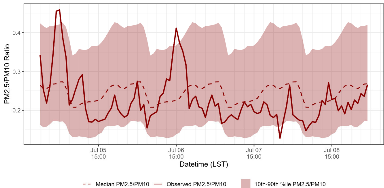
PM2.5/PM10 - Paul Meyer (320030043) 2023-07-05 to 2023-07-08
