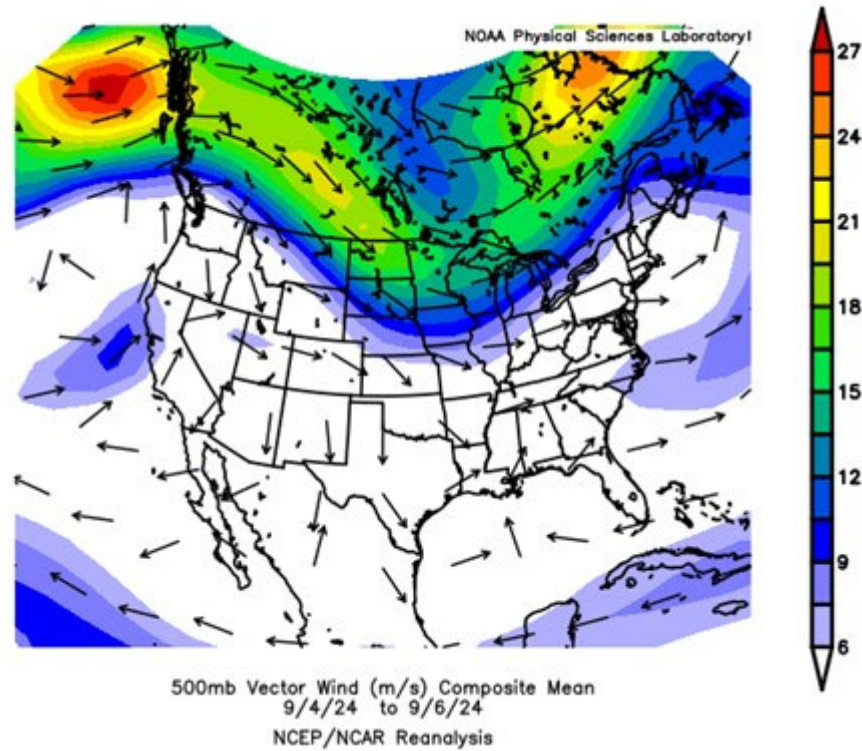
Figure 339. Mean 500-mb winds between September 4-6, 2024. Upper-level high pressure over southern Nevada and the Colorado River Valley produced light north-northeasterly winds aloft in the Clark County area. Source: NOAA.
