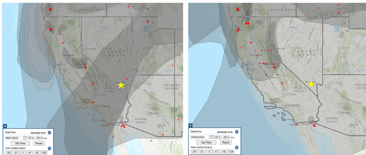
Figure 193. HMS smoke analysis from September 1, 2022 (left), and September 2 (right). The images show moderate density smoke over the Las Vegas region (star) on September 1, and light density smoke over Las Vegas on September 2. Source: AirNow-Tech
