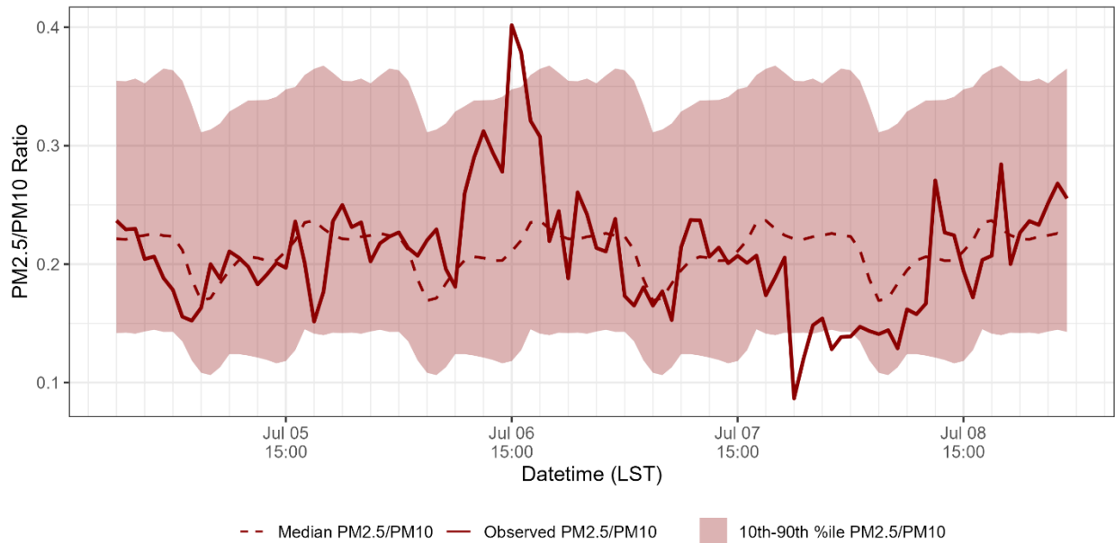
PM2.5/PM10 - Liberty High School (320030299) 2023-07-05 to 2023-07-08
