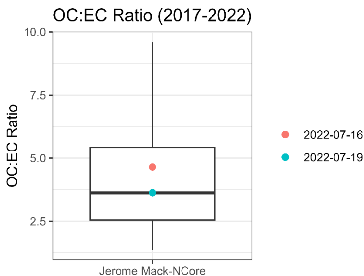
Figure 161. OC to EC ratio boxplot of ratios collected from 2017-2022 during the May-October ozone production season. Samples taken nearest to the atypical event date are displayed as points.
