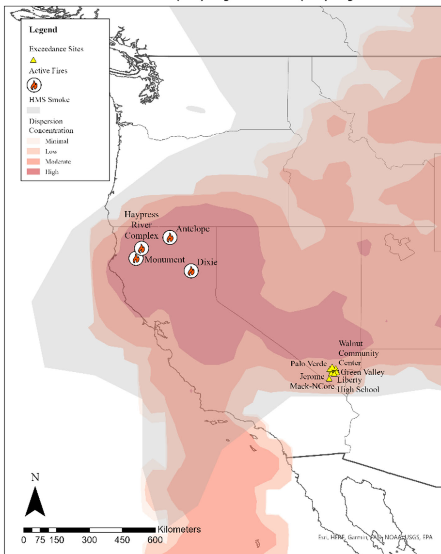
Figure 94. HYSPLIT dispersion modeling for four large fires (labeled as "Active Fires") throughout the western U.S. GDAS 1.0° meteorological data was used, and dispersion was initiated on August 5, 2021, at 16:00 PST to model the regional smoke observed in satellite and HMS products. HMS smoke is shown in gray and qualitative concentrations of particulate matter are shown in shades of red. Accumulation of particulate matter is shown at 0-100 m for 16:00 PST on August 6 through 16:00 PST on August 7, 2021.
