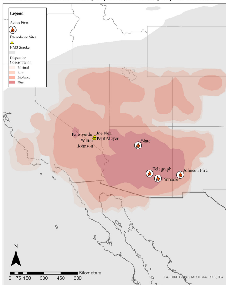
Figure 57. HYSPLIT dispersion modeling for the large fires (labeled as “Active Fires”) in Arizona and New Mexico. GDAS 1.0° meteorological data was used, and dispersion was initiated on June 6, 2021, at 00:00 PST to model the regional smoke observed in satellite and HMS products. HMS smoke is shown in gray and qualitative concentrations of particulate matter are shown in shades of red. Accumulation of particulate matter is shown in the 0-100 m vertical layer for 00:00 PST on June 16 through 00:00 PST on June 18, 2021.
