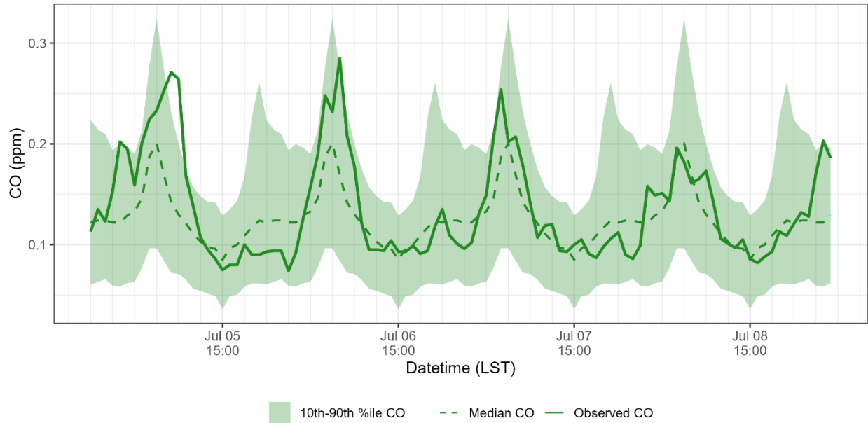
CO - Paul Meyer (320030043) 2023-07-05 to 2023-07-08
