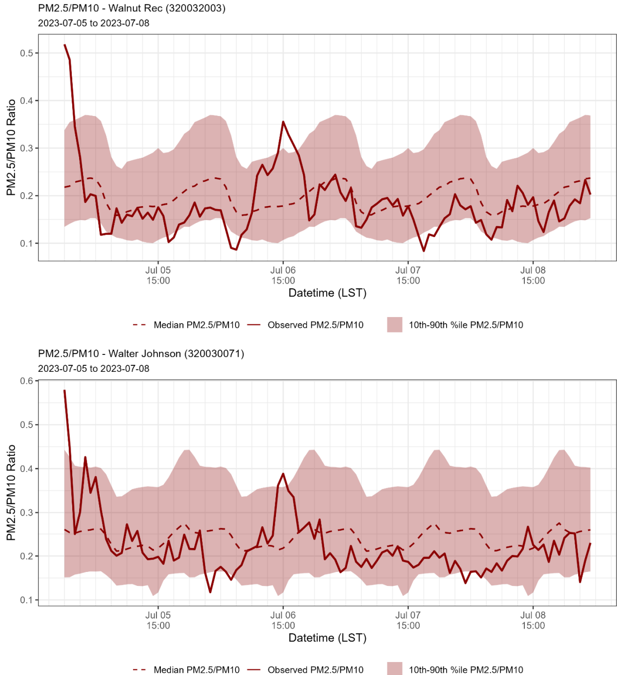
Figure 245. Ratio of PM 2.5 -to-PM 10 concentrations during the event period overlaid on the 10th to 90th percentile diurnal concentrations at Jean (AQ5 site code 320031019), Jerome Mack (AQ5 site code 320030540), Liberty (AQ5 site code 320030299), Green Valley (AQ5 site code 320030298), Joe Neal (AQ5 site code 320030075), Palo Verde (AQ5 site code 320030073), Walter Johnson (AQ5 site code 320030071), Mountain's Edge (AQ5 site code 320030044), Paul Meyer (AQ5 site code 320030043), and Walnut Recreation (AQ5 site code 320032003). The 10th to 90th percentile concentration is calculated across the ozone production season (April-September) for 2018-2023. Note: Walnut Recreation includes data from June 1, 2021, and onwards; Mountain's Edge includes data from October 1, 2020, and onwards; Liberty includes data from May 1, 2021, and onwards.
