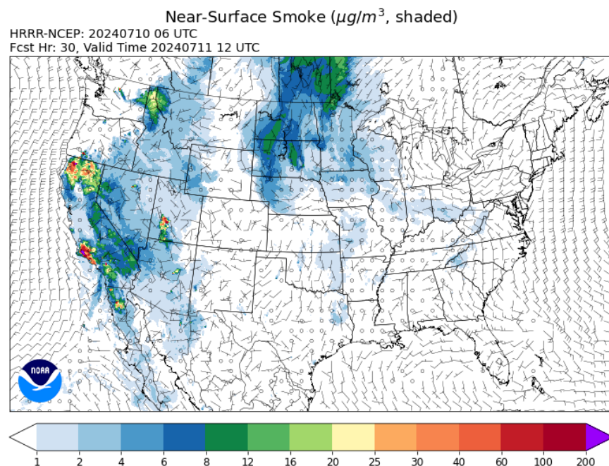
Figure 272. Model prediction (initialized 06 UTC July 10) of near-surface smoke ( \mu\text{g}/\text{m}^3 ) at 04:00 PST on July 11, 2024, showed near-surface smoke over southern Nevada. Image courtesy of NOAA's Global Systems Laboratory.
