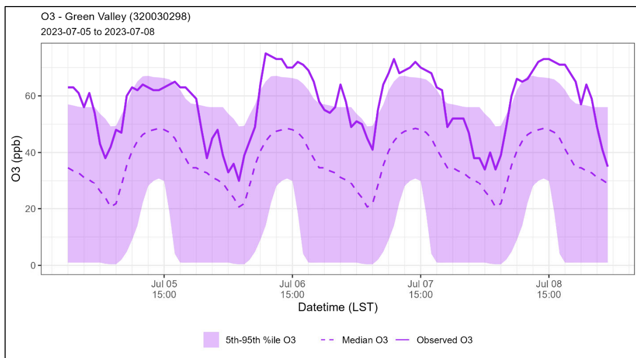
Figure 203. Hourly O 3 measurements overlaid on the 5th to 95th percentile diurnal concentration at Green Valley (AQ5 site code 320030298). The 5th to 95th percentile concentration is calculated across the ozone production season (April-September) for 2018-2023.
