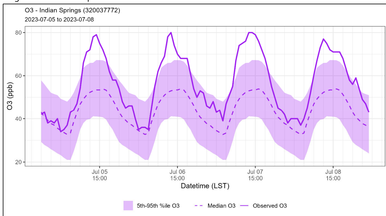
Figure 204. Hourly O 3 measurements overlaid on the 5th to 95th percentile diurnal concentration at Indian Springs (AQS site code 320037772). The 5th to 95th percentile concentration is calculated across the ozone production season (April-September) for 2018-2023.
