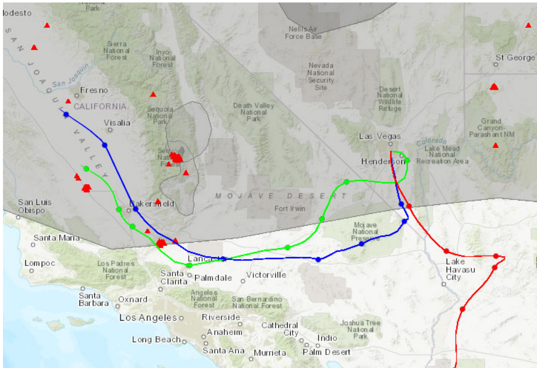
Figure 306. 48-hour back trajectory analysis (green – 10 m AGL, blue – 2,500 m AGL, red – 5,000 m AGL) ending at 11:00 PST on July 17. The 10 m AGL and 2,500 m AGL transport paths intersected a NOAA-analyzed smoke plume from July 15 and were near fires detected by satellites on July 15 in the Tehachapi Mountains. Source: AirNow-Tech.
