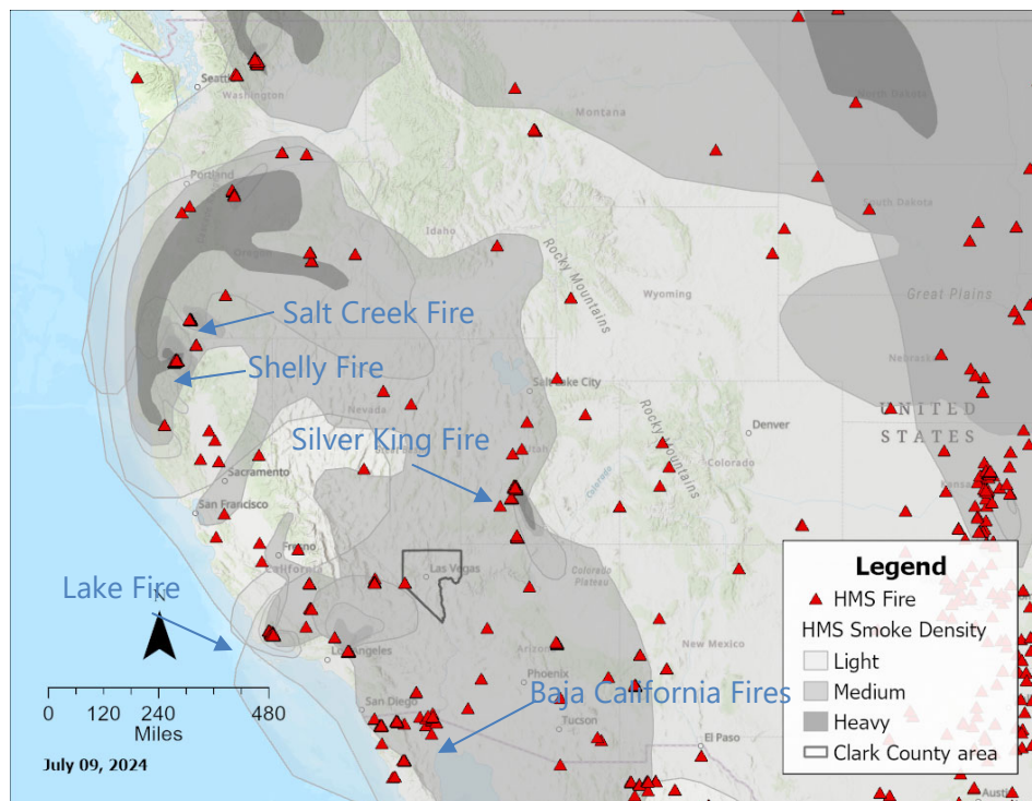
Figure 266. Western U.S. view of HMS fire detections and smoke density on July 9, 2024.
