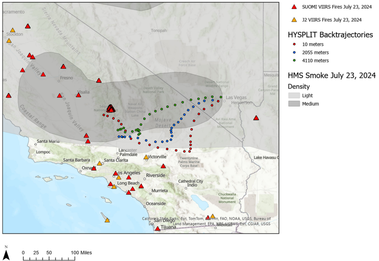
Figure 331. 24-hour boundary-layer backward trajectories from the HRRR model ending at 16:00 PST July 24, 2024, at 10 meters (red dots), 2,055 meters (blue dots) and 4,110 meters (green dots). HMS fires (triangles) and smoke (gray contours) are also displayed.
