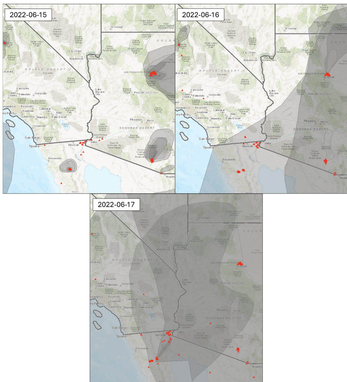
Figure 133. HMS smoke maps for June 15-17, 2022, showing fire and smoke detections in southern CA, NV, AZ, and Baja Mexico. Smoke is shown as gray shades on top of the map with darker gray indicating denser smoke plumes. Fire detections are shown as red triangles.
