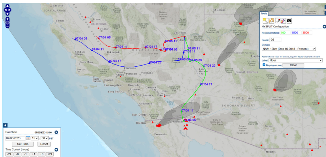
Figure 224. 36-hr back trajectory from the NAM model ending in Las Vegas on July 5, 2023, at 15:00 PST at 100 m (green line), 1,500 m (blue line), and 3,500 m (red line) HMS fires (triangles) and smoke (gray shading) on July 5 are also displayed. Image courtesy of EPA's AirNow-Tech.
