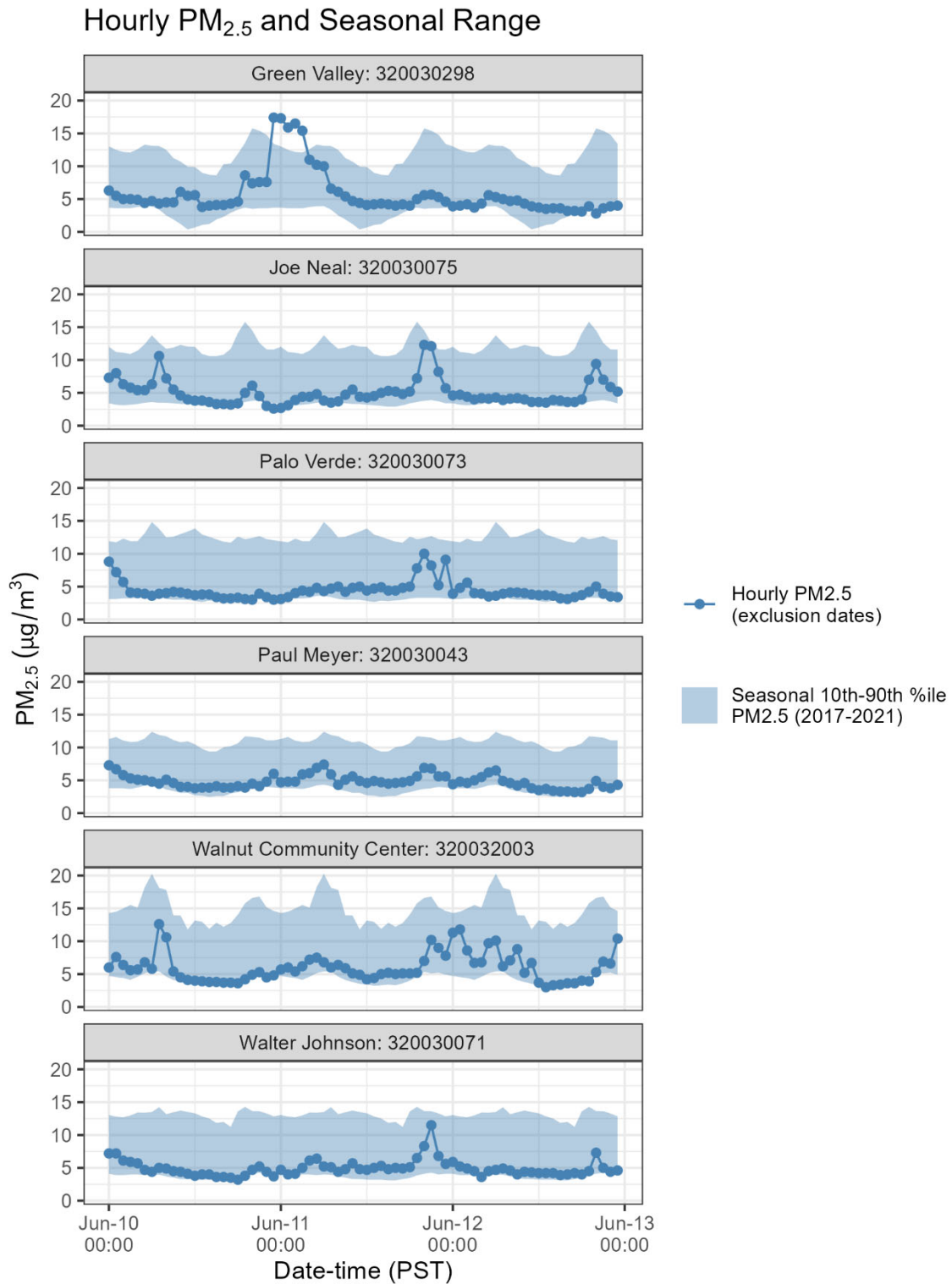
Figure 50. Hourly PM 2.5 measurements overlaid on the 10th-90th percentile diurnal concentration at all affected sites.
