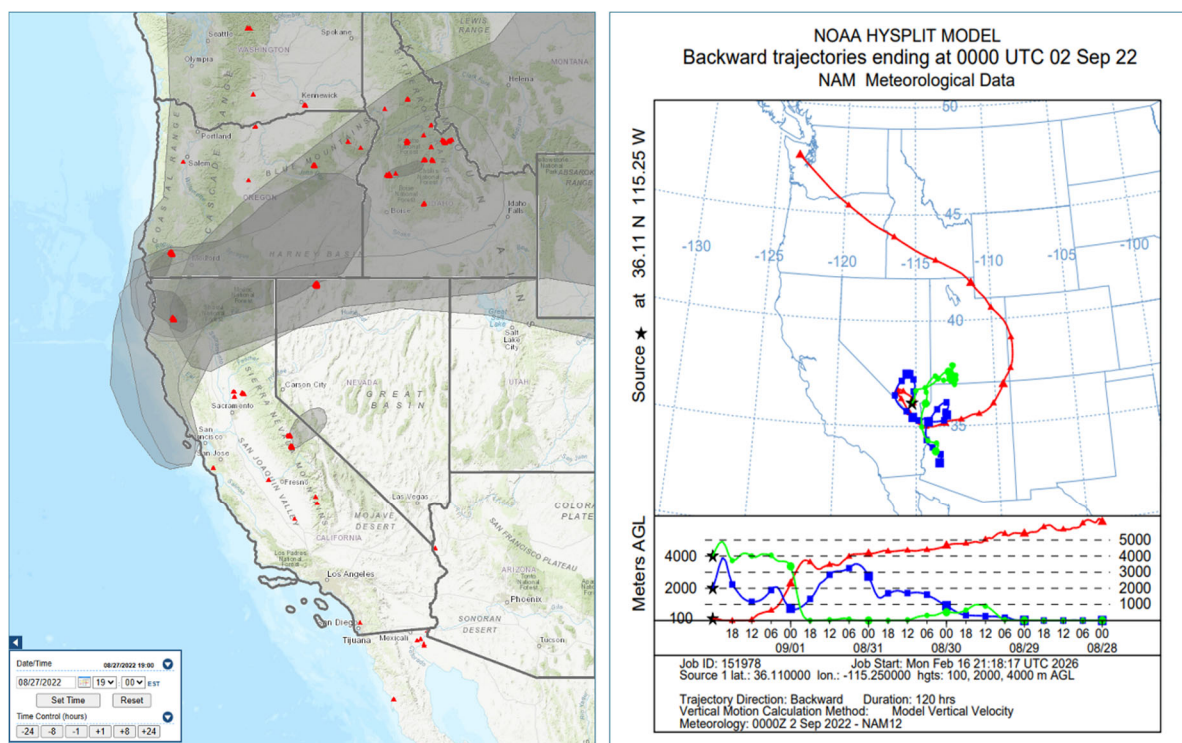
Figure 192. (Left) HMS smoke analysis from August 27, 2022 (120 hours prior to the September 1, 2022 exceedance). (Right) 120-hour NAM 12-km HYSPLIT back trajectories at 100 m (red), 2,000 m (blue), and 4,000 m (green), initiated at 16:00 PST on September 1 (00 UTC September 2) at the Paul Meyer air quality monitor. Sources: EPA's AirNow-Tech and NOAA's Air Resources Laboratory.
