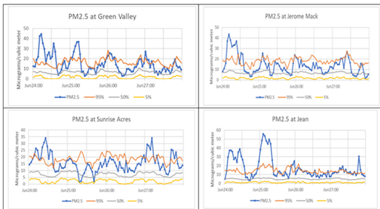
Figure 15. 6-yr hourly seasonal 95th, 50th, and 5th percentiles for PM 2.5 concentrations ( \mu\text{g}/\text{m}^3 ) at LVV FEM monitors during June 24-27, 2016.
