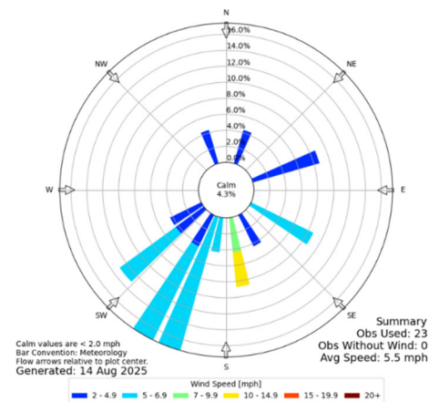
Windrose Plot for [LAS] Las Vegas - Harry Reid Intl Obs Between: 15 Jul 2024 10:56 PM - 16 Jul 2024 11:56 PM America/Los_Angeles
