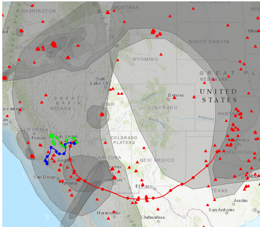
Figure 303. 72-hour back trajectory analysis (green – 50 m AGL, blue – 2,100 m AGL, red – 4,200 m AGL) ending at 16:00 PST on July 15. The 4,200 m AGL path intersects NOAA-analyzed smoke (grey contours) and is near fires (red triangles) detected by satellites on July 12. Source: AirNow-Tech.
