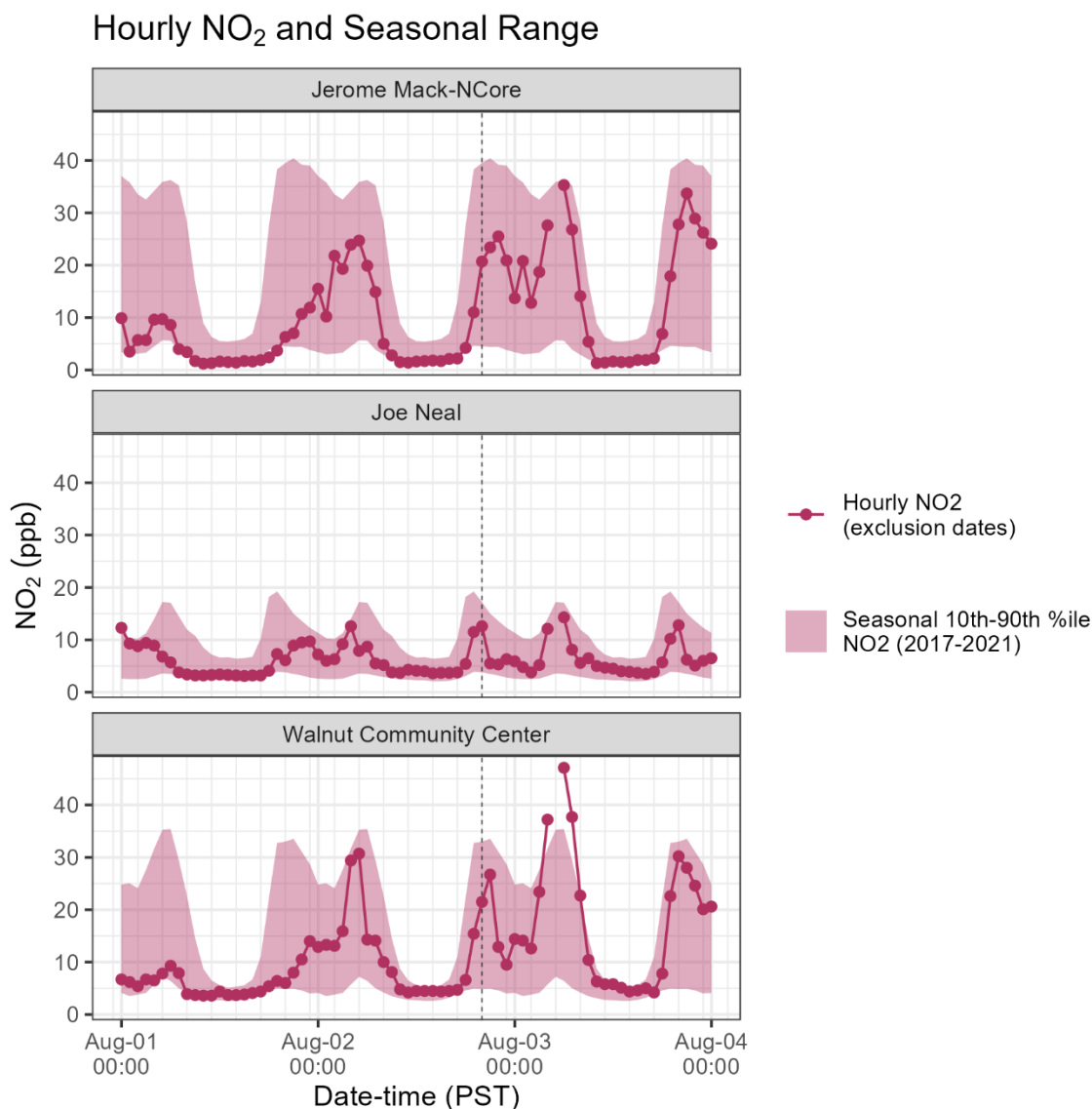
Figure 89. Hourly NO 2 measurements overlaid on the 10th-90th percentile diurnal concentration at affected sites. The 10th-90th percentile concentration is calculated across the ozone production season (May-October) of 2017-2021. The dashed line is August 2, 2021, at 20:00 PST.
