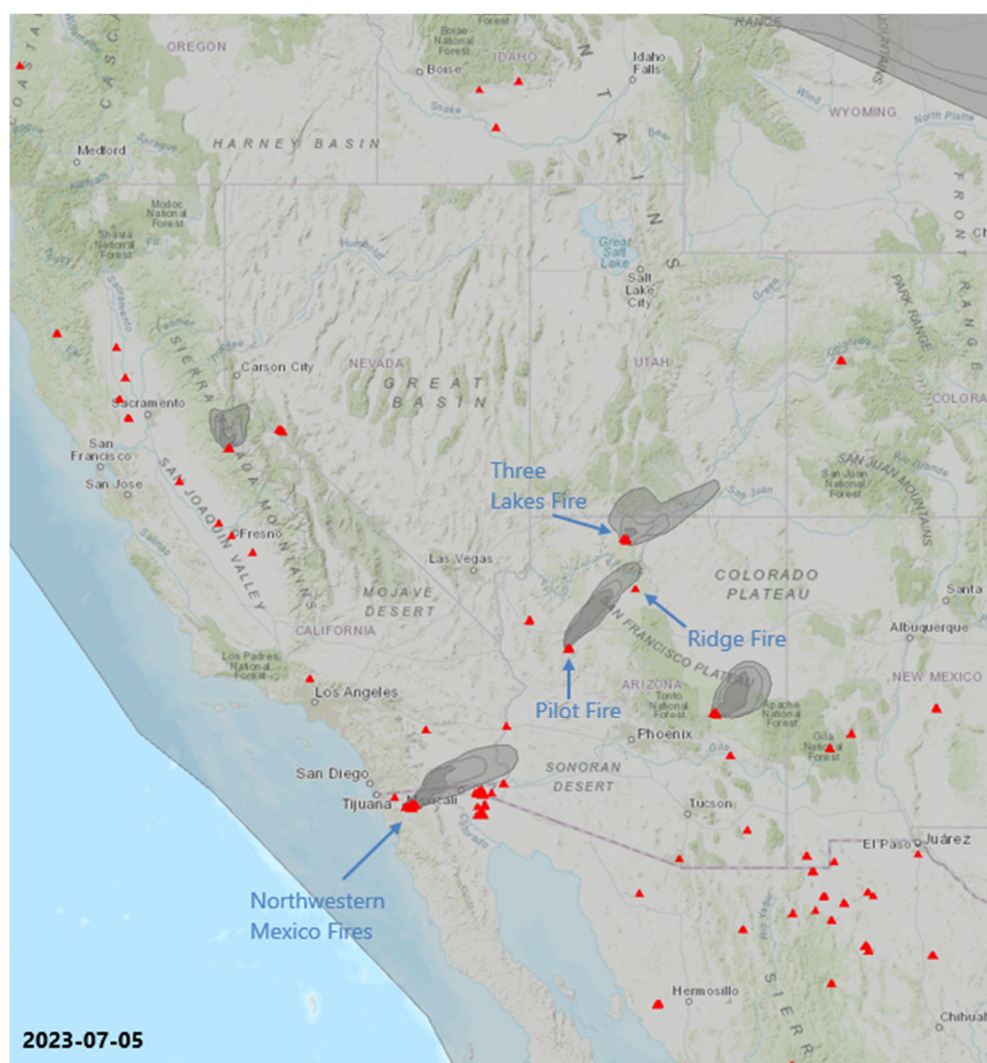
Figure 214. NOAA HMS smoke analysis (grey contours) and satellite fire detections (red triangles) for July 5, 2023. Source: AirNow-Tech.
