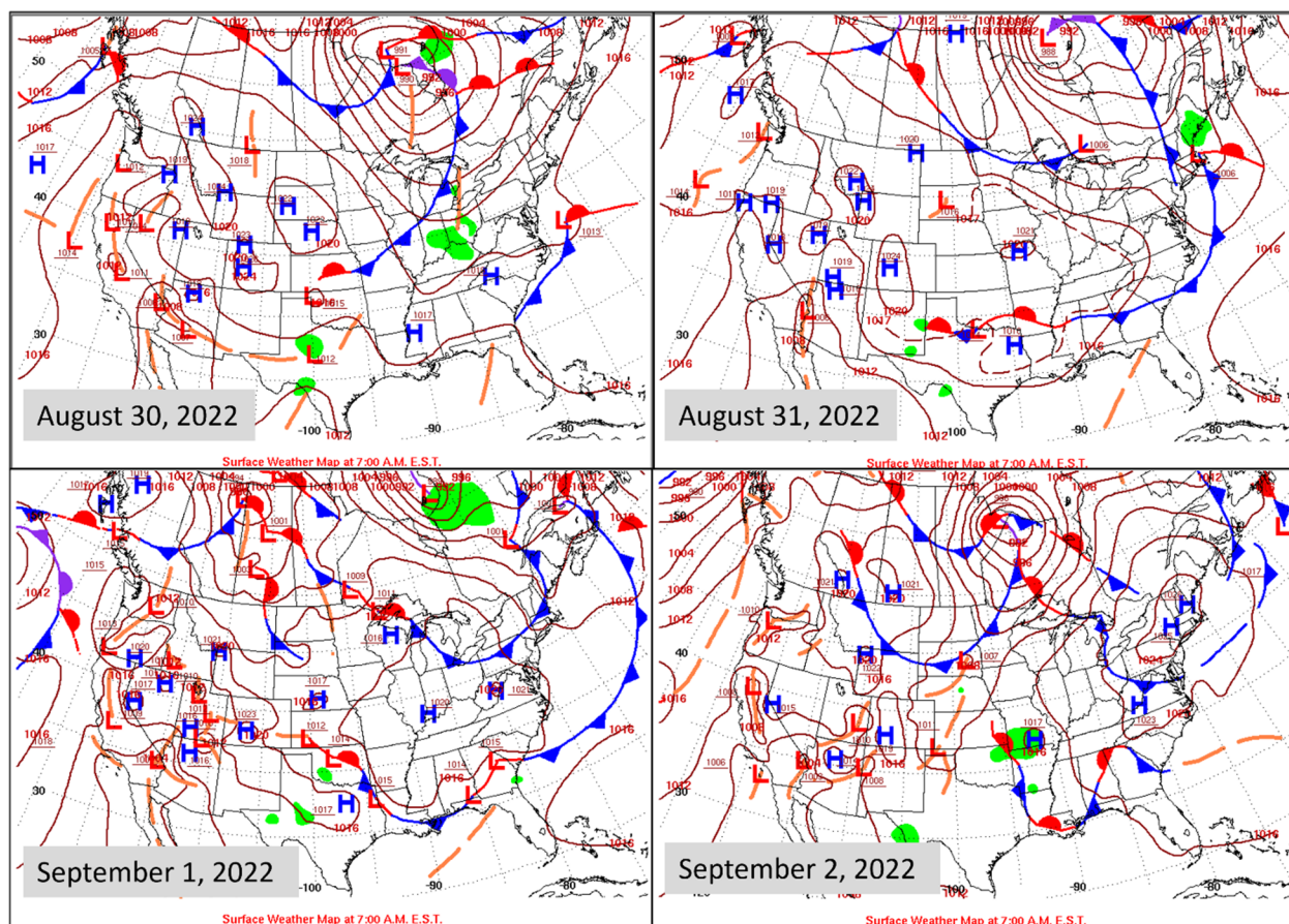
Figure 182. Daily surface-level weather maps for August 30-September 2, 2022. Source: NOAA's Weather Prediction Center
