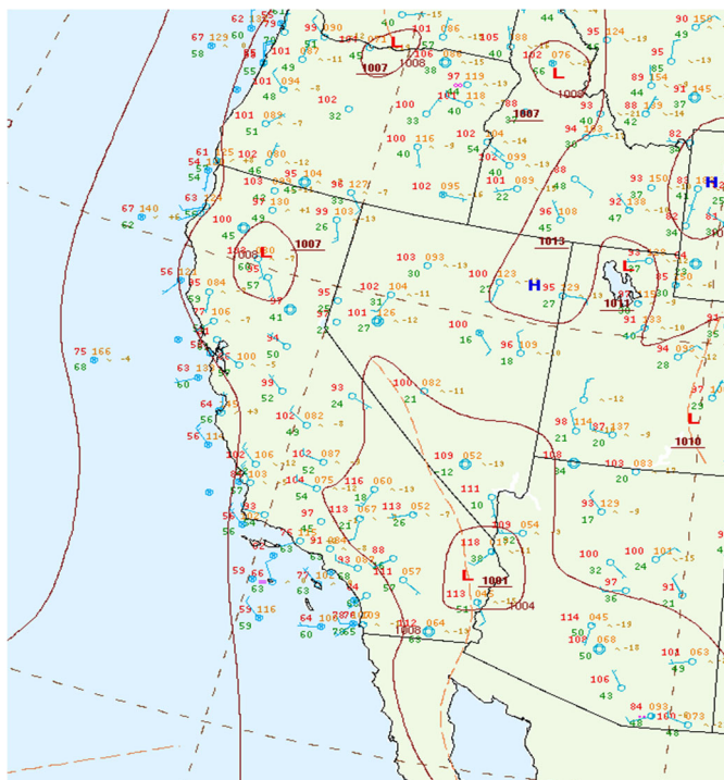
Figure 278. Surface weather conditions at 13:00 PST on July 9, 2024. Image courtesy of NOAA's Weather Prediction Center.
