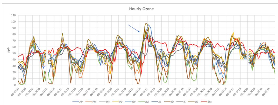
Figure 12. Time series of 1-hr ozone (ppb) at all LVV monitors during June 20-28, 2016.
