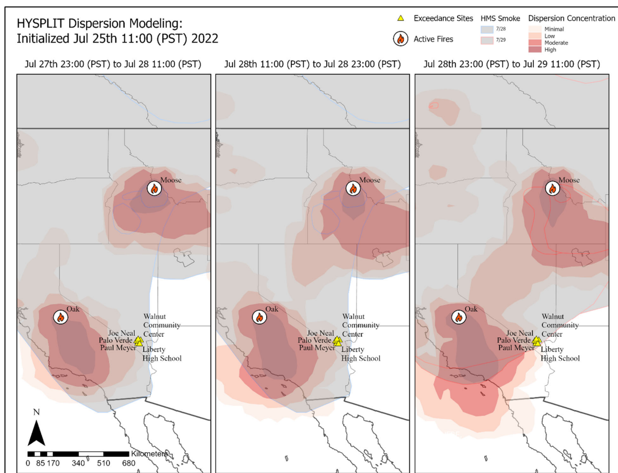
Figure 173. HYSPLIT dispersion modeling for two large fires (labeled as “Active Fires”) in California and Idaho on or before the exclusion dates of July 28-29, 2022. GDAS 1.0° meteorological data was used, and dispersion was initiated on July 25 at 11:00 PST to model the regional smoke transport. HYSPLIT-modeled qualitative concentrations of particulate matter are shown in shades of red, and independently sourced HMS satellite-detection smoke plumes are shown in gray. HYSPLIT accumulation of particulate matter is shown at 0-2,600 m.
