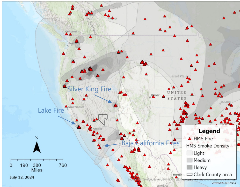
Figure 269. Continental view of HMS fire detections and smoke density on July 12, 2024.
