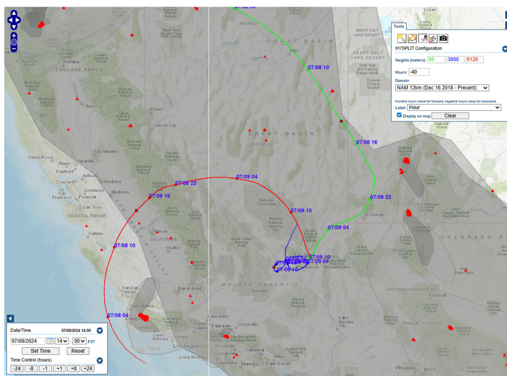
Figure 281. 40-hr boundary-layer back trajectories from the NAM model ending in Las Vegas at 15:00 PST on July 9, 2024, at 50 m (green line), 3,000 m (blue line), and 6,120 m (red line). HMS fires (triangles) and smoke (gray shading) on July 8 are also displayed. Image courtesy of EPA's AirNow-Tech.
