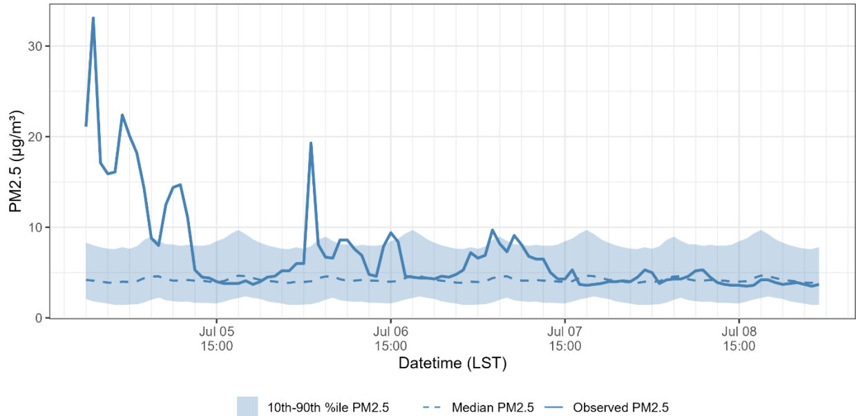
PM2.5 - Palo Verde (320030073) 2023-07-05 to 2023-07-08
