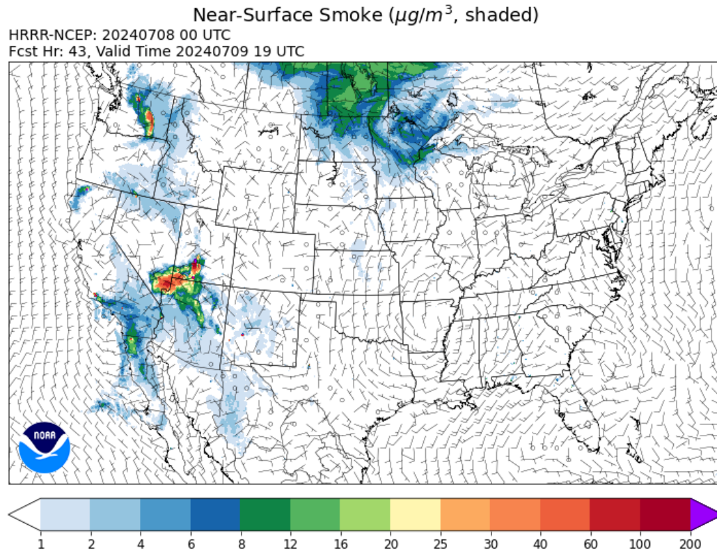
Figure 270. Model prediction (initialized 00 UTC July 8) of near-surface smoke ( \mu\text{g}/\text{m}^3 ) at 11:00 PST on July 9, 2024, showed near-surface smoke over southern Nevada. Image courtesy of NOAA's Global Systems Laboratory.
