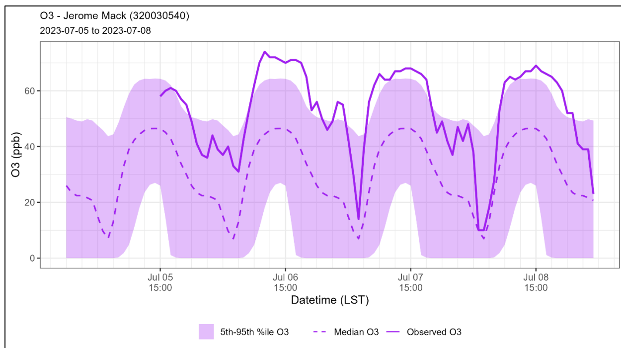
Figure 206. Hourly O 3 measurements overlaid on the 5th to 95th percentile diurnal concentration at Jerome Mack (AQ5 site code 320030540). The 5th to 95th percentile concentration is calculated across the ozone production season (April-September) for 2018-2023.
