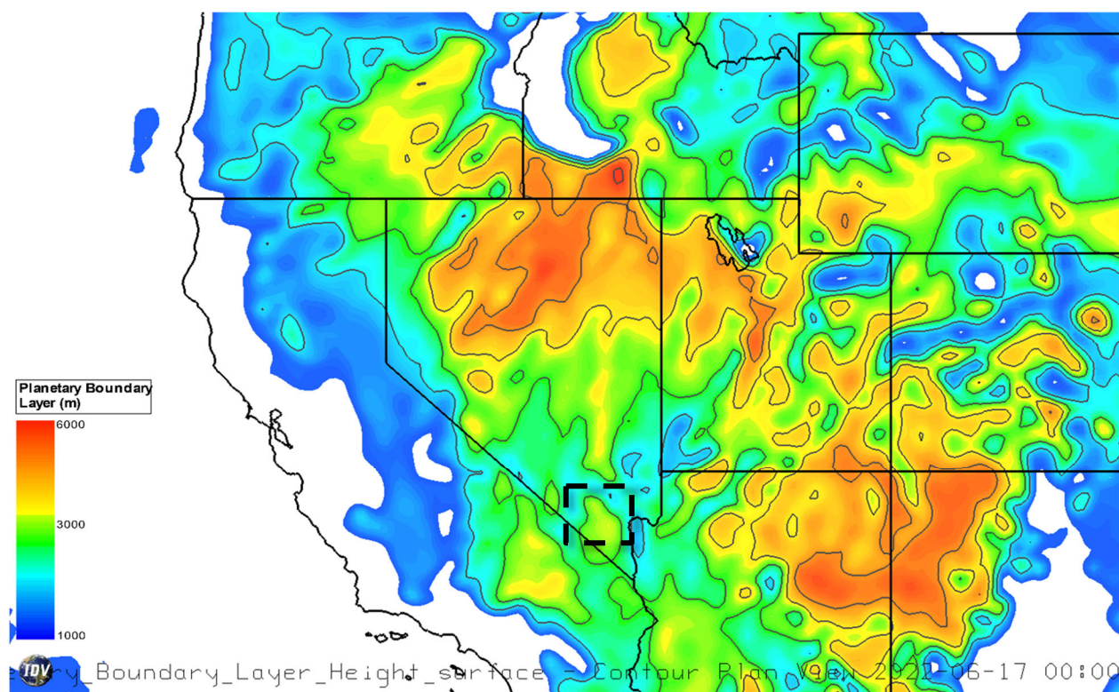
Figure 136. PBL height contour map based on the NAM model for June 17, 2022, at 00:00 UTC (June 16 at 16:00 PST). The gray lines denote PBL heights above 2,000 m in altitude in 1,000 m increments. Color contours begin at 1,000 m AGL. Clark County, NV, is enclosed by a dashed, black box.
