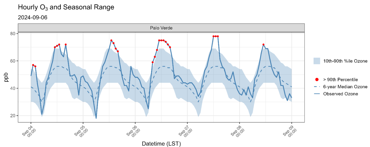
Figure 337. Hourly ozone concentrations (ppb) for September 6, 2024, and surrounding days compared to 6-year ozone season (April 1 – September 30) hourly medians and 10th-to-90th percentiles.
