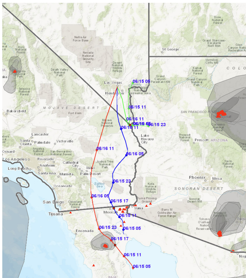
Figure 134. 36-hour HYSPLIT backward trajectory analysis starting on June 16, 2022, at 14:00 PST and NOAA HMS smoke analysis (grey shading) and satellite fire detections (red triangles) on June 15. HYSPLIT shows air advection from Baja Mexico fires into Clark County by June 16, 2022, using NAM 12 km meteorological data. Forward trajectory heights were modeled at 100 m (green), 1,850 m (blue), and 3,600 m (red) AGL to show near-surface and synoptic flow.
