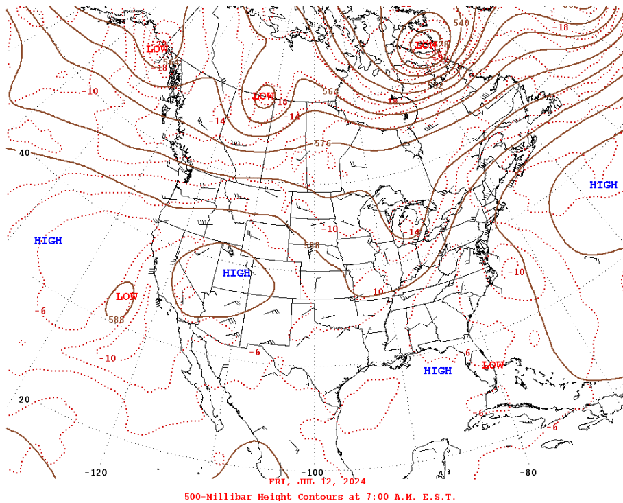
Figure 277. 500-mb heights, winds, and temperatures at 04:00 PST on July 12, 2024. Image courtesy of NOAA's Weather Prediction Center.
