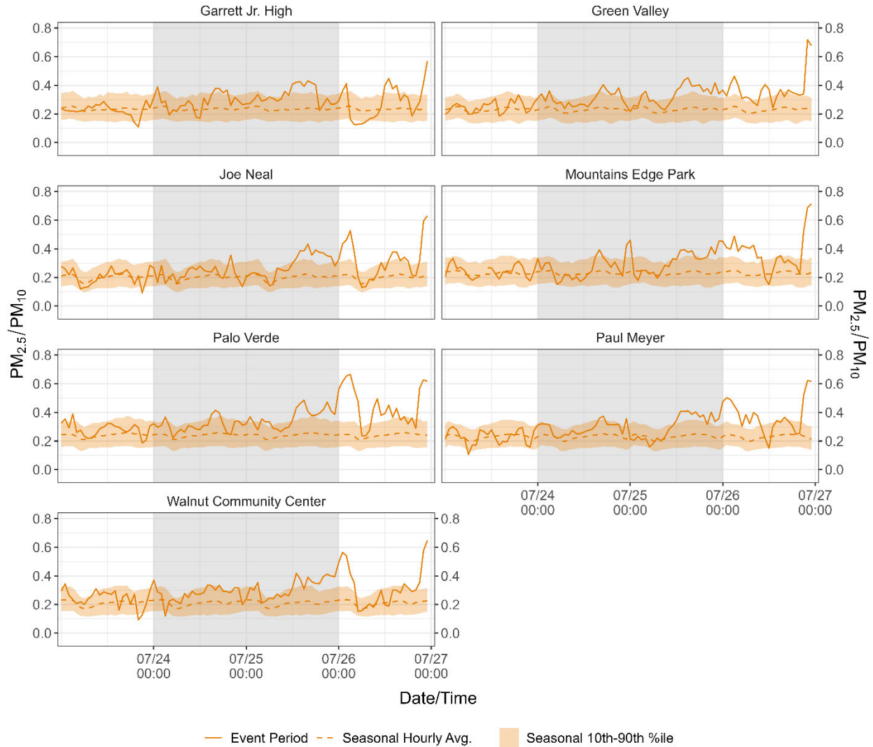
Figure 336. Ratio of PM_{2.5} -to- PM_{10} concentrations during the event period, overlaid on the 10th-to-90th percentile diurnal concentrations at the Garrett Jr. High* (AQS site code 320030602), Green Valley (AQS site code 320030298), Joe Neal (AQS site code 320030075), Mountain's Edge* (AQS site code 320030044), Palo Verde (AQS site code 320030073), Paul Meyer (AQS site code 320030043), and Walnut Community Center* (AQS site code 320032003) sites. The 10th-to-90th percentile concentration is calculated across the ozone production season (April-September) of 2019-2024. Note: the Apex site only includes data from June 1, 2023, and onwards; the Garrett Jr. High site only includes data from April 1, 2021, and onwards; the Mountain's Edge site only includes data from October 1, 2020, and onwards; and the Walnut Community Center site only includes data from June 1, 2021, and onwards.
