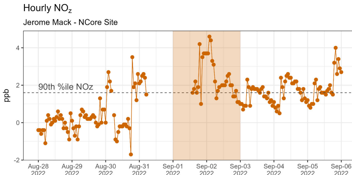
Figure 199. Hourly NO z (i.e., NO y -NO x ) concentrations at the Jerome Mack site for the September 1-2 event days and three days before and after the event. The 90th percentile of 2017-2022 NO z concentrations is shown as the dashed line. The event day is highlighted in orange.
