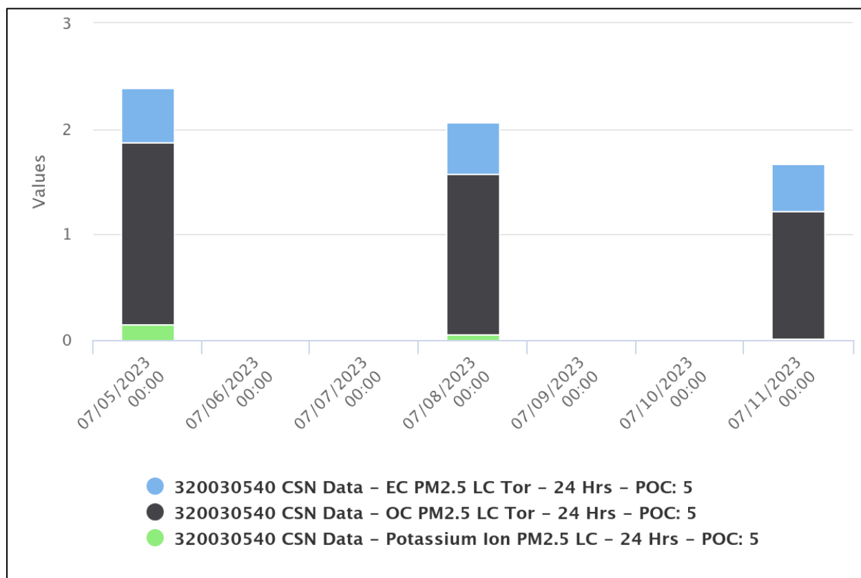
Figure 244. PM 2.5 speciation filter data from Jerome Mack CSN on July 5, 8, and 11 2023 for wildfire smoke tracers, elemental carbon (EC), organic carbon (OC), and potassium (K + ).
