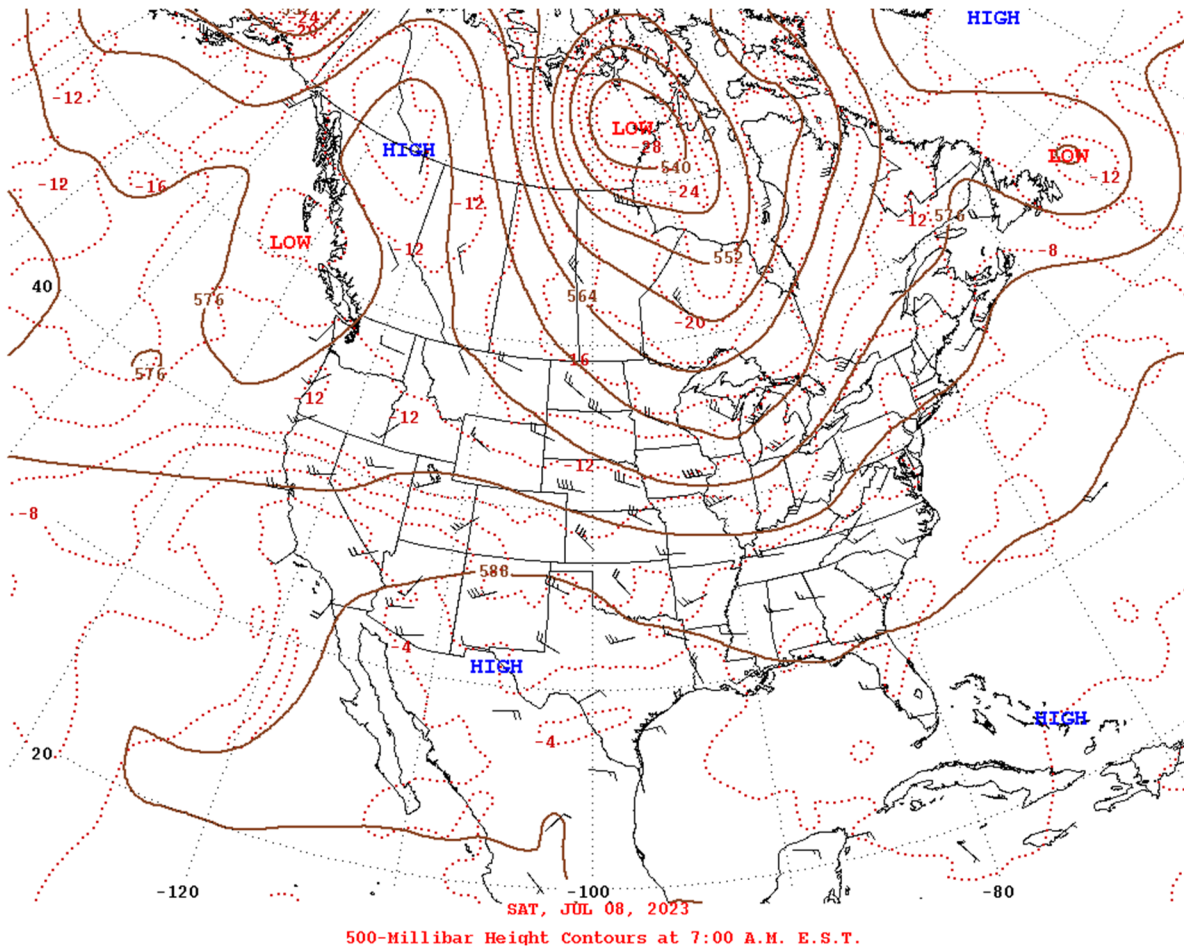
Figure 222. 500-mb heights, winds, and temperatures at 7:00 A.M. E.S.T. Source: NOAA Weather Prediction Center.
