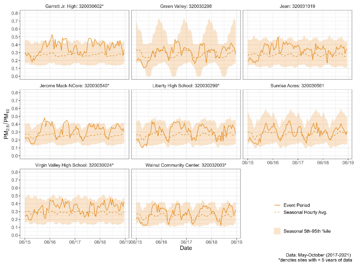
Figure 67. Ratio of PM_{2.5} -to- PM_{10} concentrations at the non-affected sites during the June 16 and June 17 event period. The 5-yr average PM_{2.5} -to- PM_{10} diurnal ratio is displayed as a dotted line, and the 5th-95th percentile range is shown as a shaded ribbon. The 5th-95th percentile concentration range is calculated across the ozone production season (May-October) of 2017-2021.
