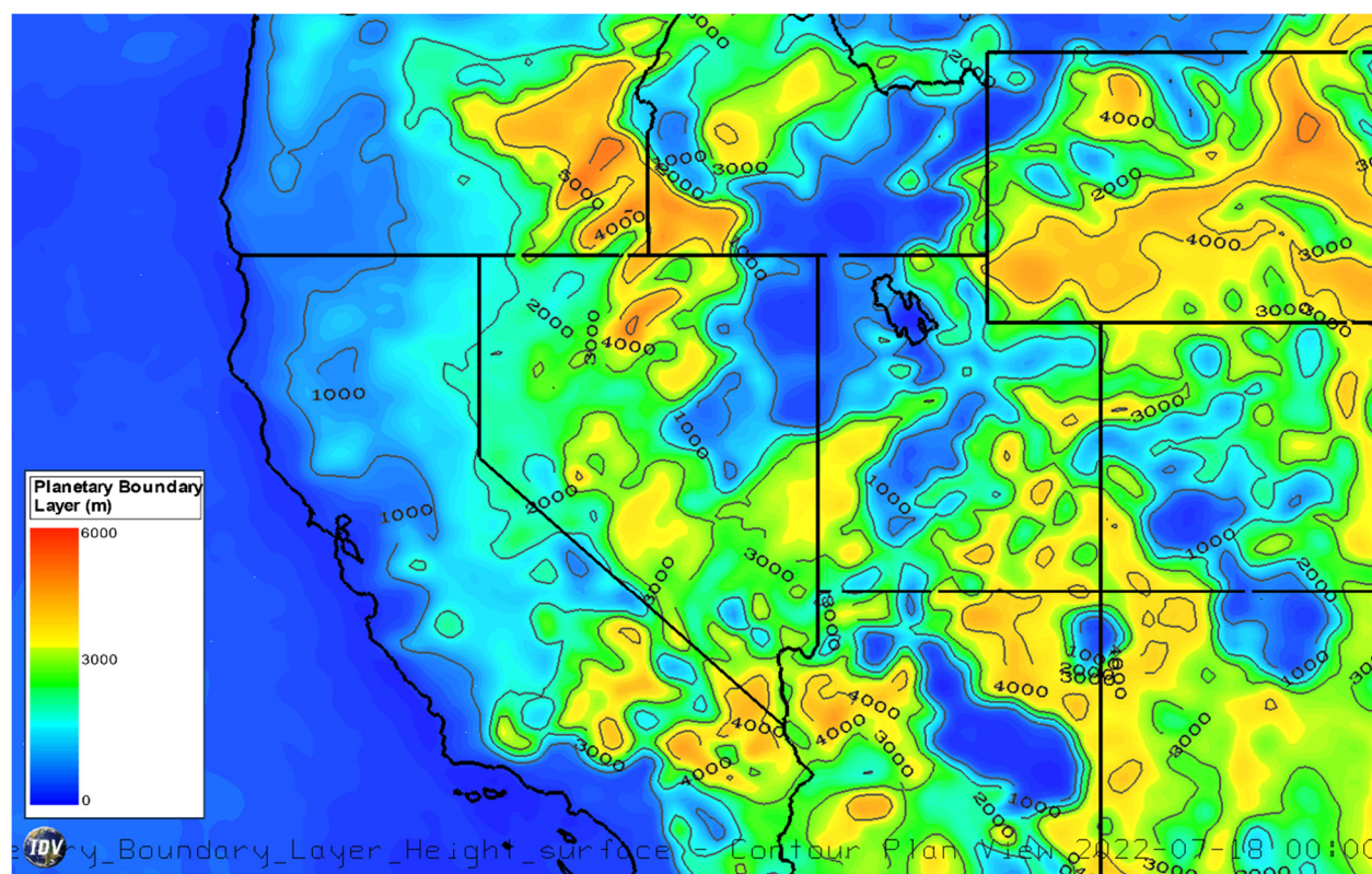
Figure 152. PBL height contour map based on the NAM model for July 18 at 00:00 UTC (July 17 at 16:00 PST). The gray lines denote PBL heights above 1 km in altitude in 1 km increments. Color contouring starts at 0 km.
