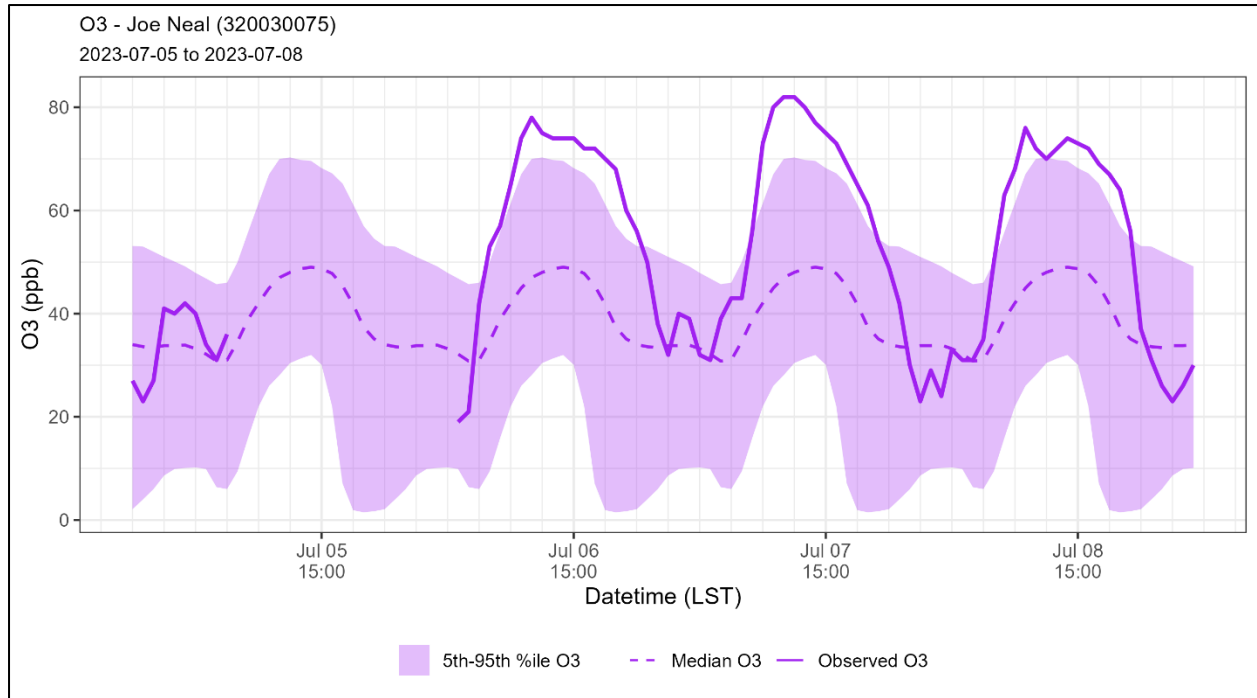
Figure 207. Hourly O 3 measurements overlaid on the 5th to 95th percentile diurnal concentration at Joe Neal (AQS site code 320030075). The 5th to 95th percentile concentration is calculated across the ozone production season (April-September) for 2018-2023.
