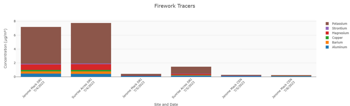
Figure 243. PM 2.5 firework tracer filter data for Jerome Mack and Sunrise Acres on July 4 and 5, 2023 from DRI. PM 2.5 firework tracer filter data for Jerome Mack on July 5 and 8, 2023 from CSN.
