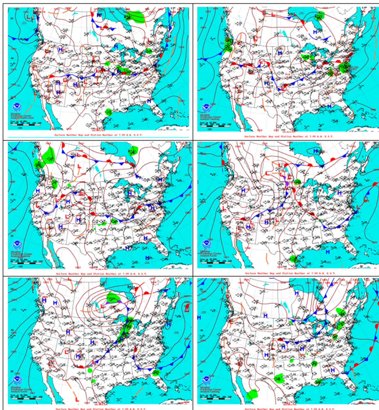
Figure 9. Surface weather patterns at 07:00 EST (04:00 PST) from June 22 to 27, 2016.
