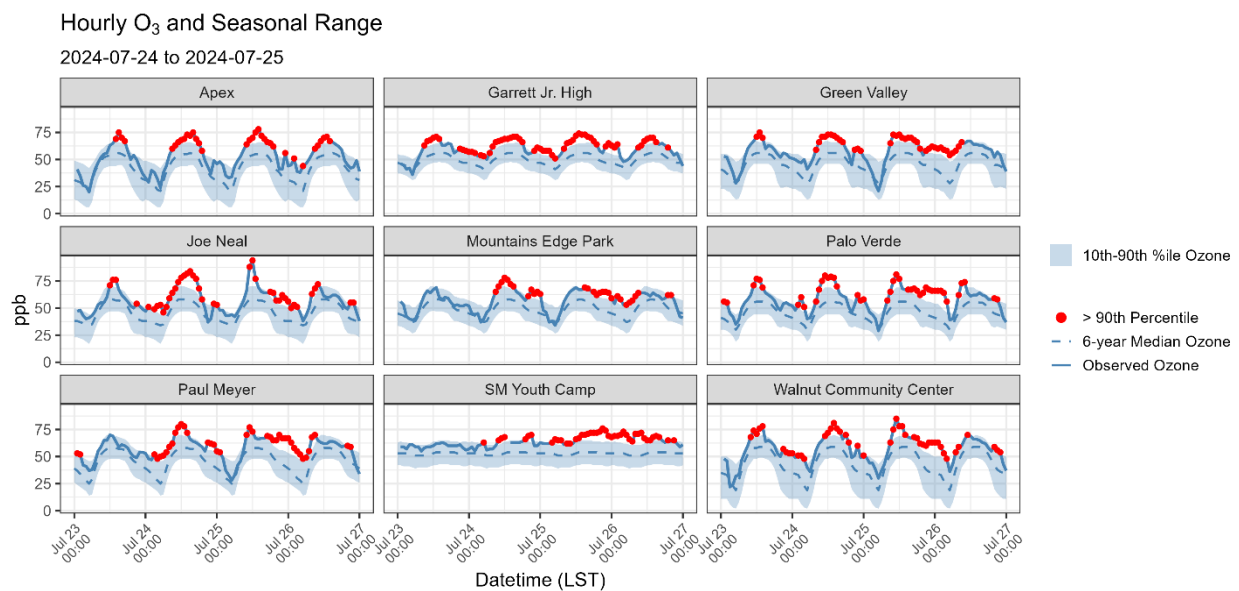
Figure 316. Hourly ozone concentrations (ppb) compared to 6-year ozone season (April 1 – September 30) hourly medians and 10th-to-90th percentiles. Note: the Apex site only includes data from June 1, 2023, and onwards; the Garrett Jr. High site only includes data from April 1, 2021, and onwards; the Mountain's Edge site only includes data from October 1, 2020, and onwards; and the Walnut Community Center site only includes data from June 1, 2021, and onwards.
