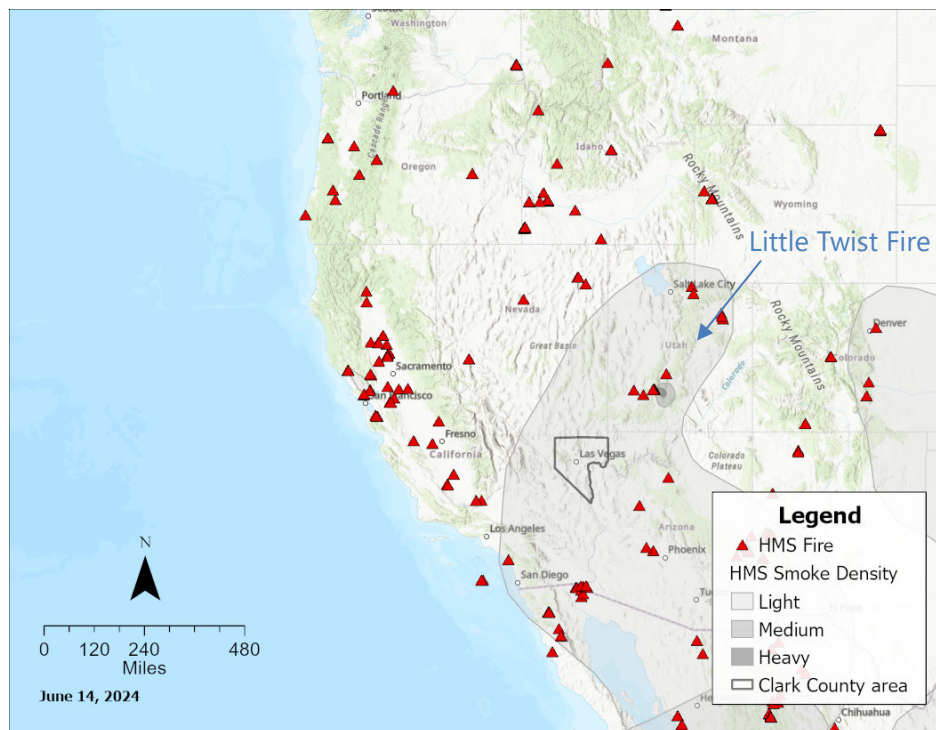
Figure 250. Western U.S. view of HMS fire detections (red triangles) and smoke density (grey contours) from June 14, 2024.
