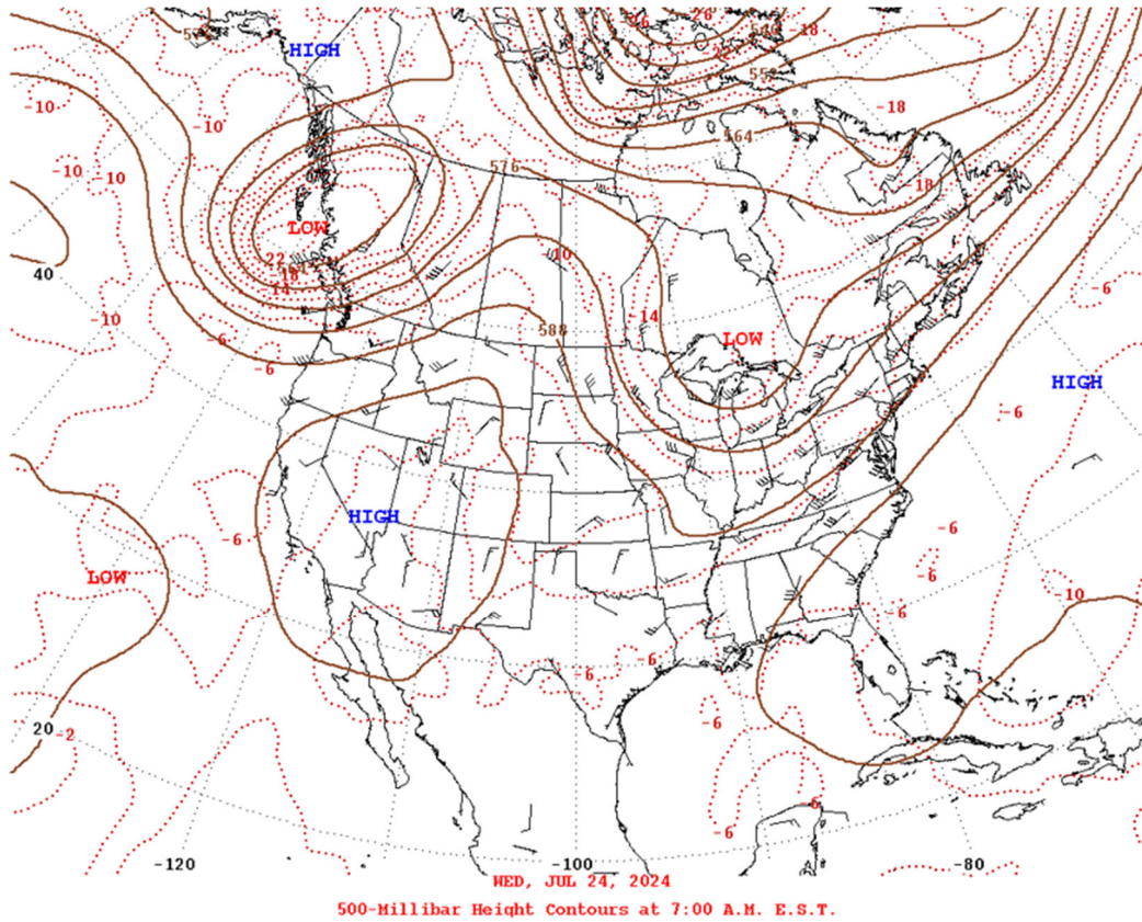
Figure 322. 500-mb heights, winds, and temperatures at 04:00 PST on July 24, 2024. Source: NOAA Weather Prediction Center.
