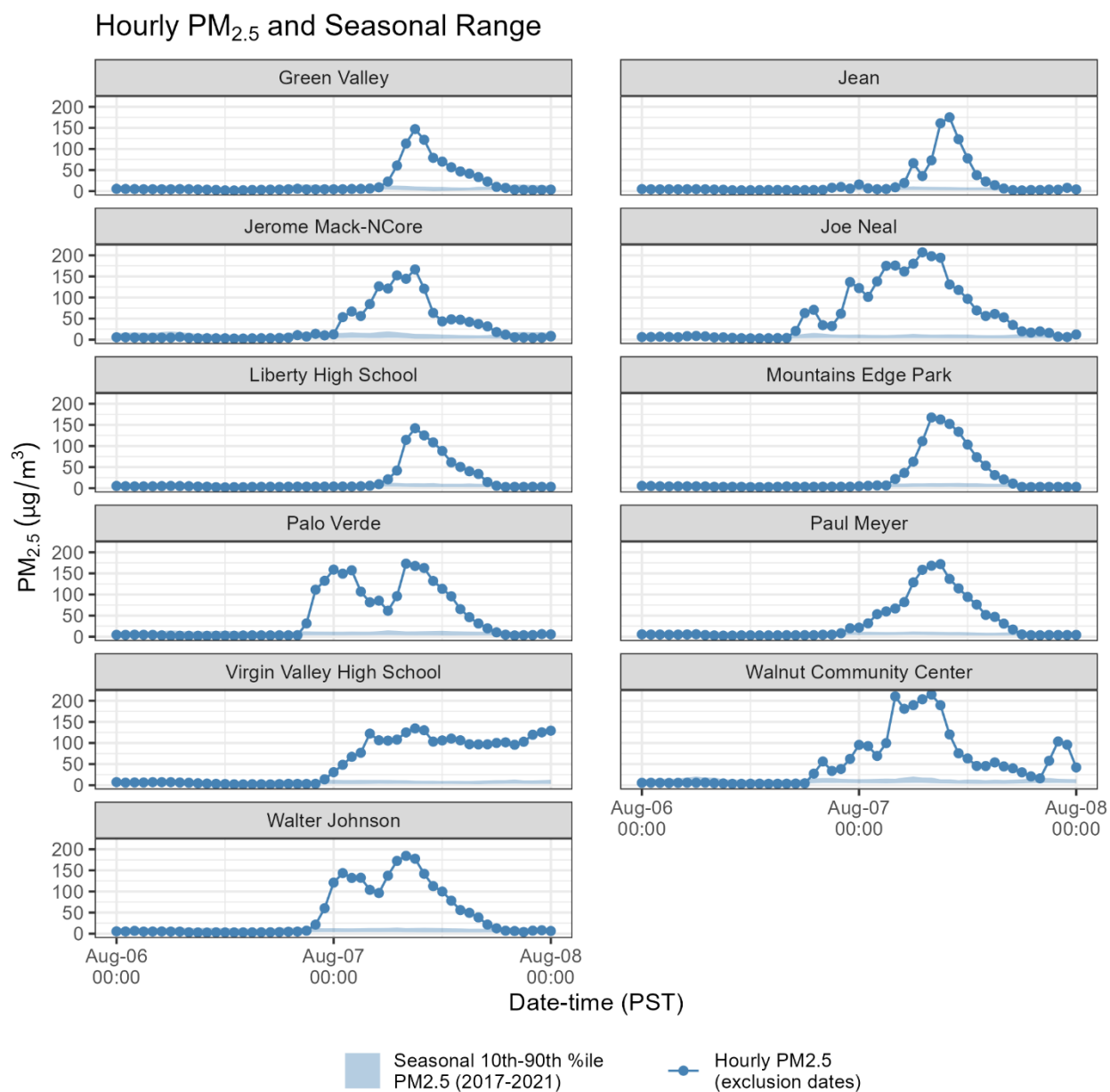
Figure 98. Hourly PM 2.5 measurements overlaid on the 10th-90th percentile diurnal concentration at affected sites that measure PM 2.5 . The 10th-90th percentile concentration is calculated across the ozone production season (May-October) of 2017-2021.
