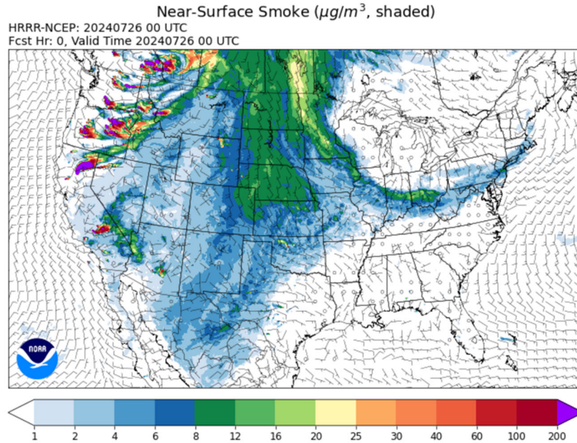
Figure 321. Model initialization of near-surface smoke ( \mu\text{g}/\text{m}^3 ) at 16:00 PST on July 25, 2024, showing near-surface smoke increasing over southern Nevada. Source: NOAA Global Systems Laboratory.
