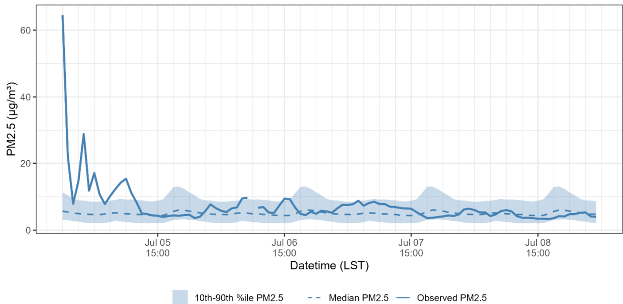
PM2.5 - Walter Johnson (320030071) 2023-07-05 to 2023-07-08
