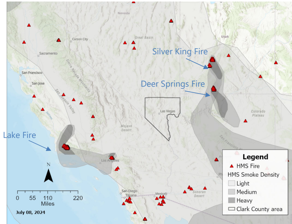
Figure 265. Regional view of HMS fire detections (red triangles) and smoke density (grey contours) on July 8, 2024.
