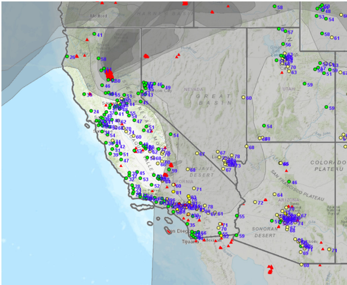
Figure 327. HMS smoke (gray contours), fire detections (red triangles), and hourly ozone concentrations (ppb) at 13:00 PST on July 25, 2024. Source: EPA AirNow-Tech.
