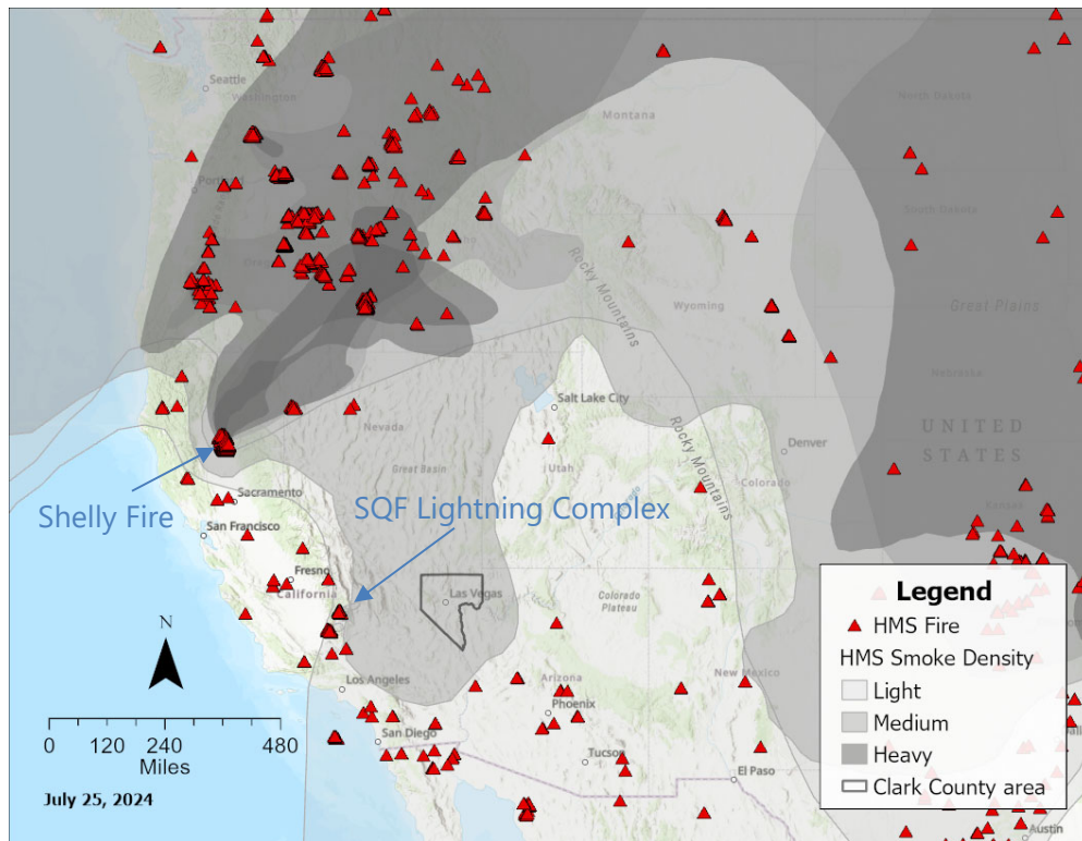
Figure 319. Western U.S. view of HMS fire detections (red triangles) and smoke density (grey contours) on July 25, 2024. Clark County is outlined in grey.
