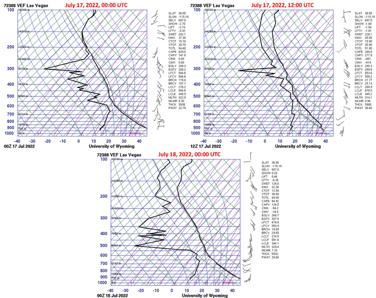
Figure 151. Skew-T soundings launched from KVEF from July 17, 2022, at 00:00 UTC (July 16 at 16:00 PST) (top left) to July 18 at 00:00 UTC (July 17 at 16:00 PST) (bottom right).
