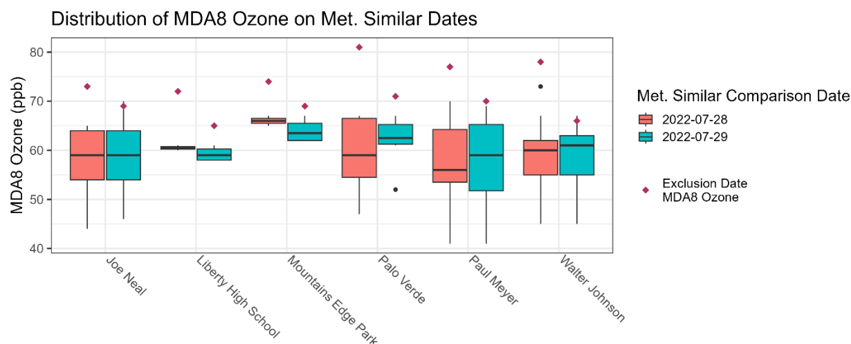
Figure 179. Distribution of MDA8 ozone concentrations on meteorologically similar days at measurement sites that were in exceedance during the exclusion period of July 28 (pink boxes) and July 29, 2022 (green boxes). MDA8 ozone concentrations measured on each exclusion date at each site are plotted as red diamonds.
