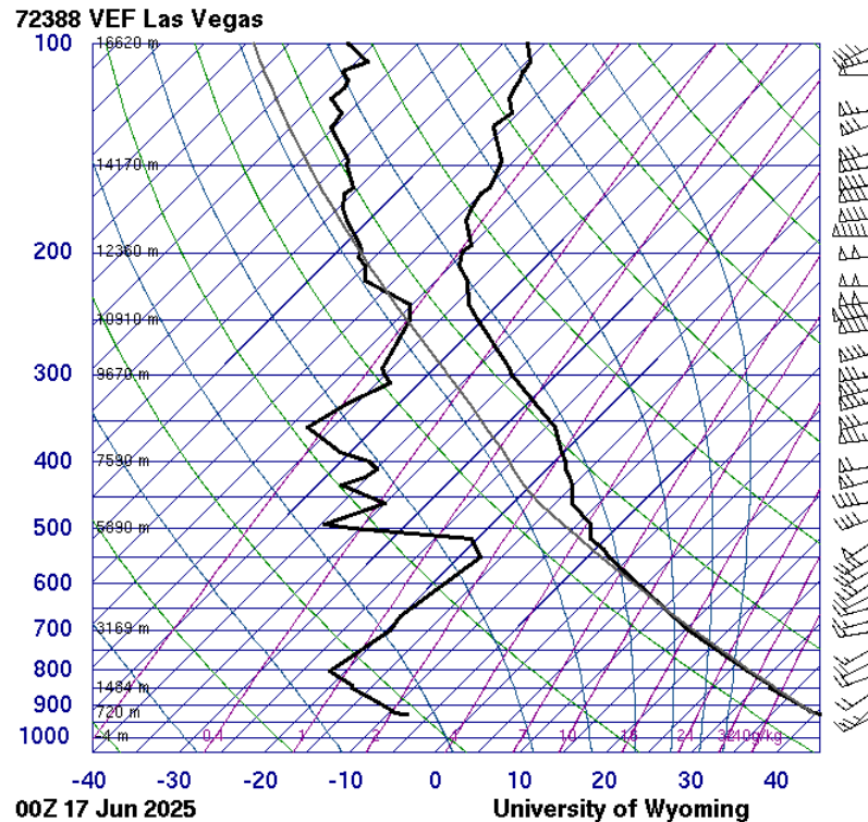
Figure 256. Observed soundings at 16:00 PST on June 16. Images courtesy of the University of Wyoming.
