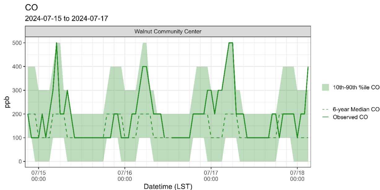
Figure 313. Hourly CO measurements overlaid on the 10th-to-90th percentile diurnal concentration at Walnut Community Center* (AQ5 site code 320032003). The 10th-to 90th percentile concentration is calculated across the ozone production season (April-September) for 2021-2024. Note: the Walnut Community Center only includes data from June 1, 2021, and onwards.
