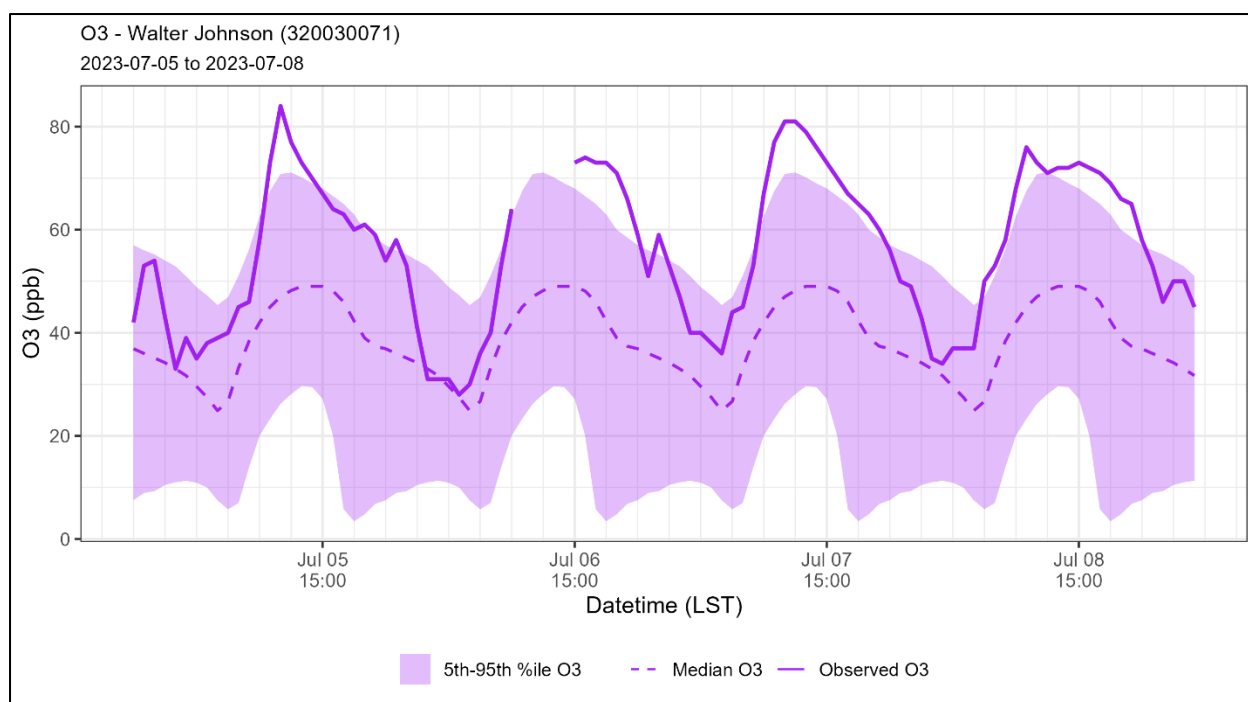
Figure 213. Hourly O 3 measurements overlaid on the 5th to 95th percentile diurnal concentration at Walter Johnson (AQ5 site code 320030071). The 5th to 95th percentile concentration is calculated across the ozone production season (April-September) for 2018-2023.
