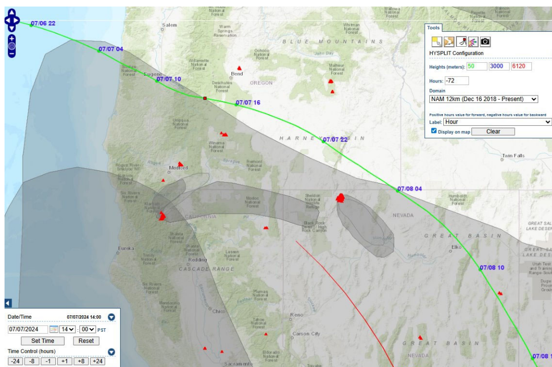
Figure 282. 72-hr boundary-layer back trajectories from the NAM model ending in Las Vegas at 15:00 PST on July 9, 2024, at 50 m (green line), and 6,120 m (red line). HMS fires (triangles) and smoke (gray shading) on July 7 are also displayed. Image courtesy of EPA's AirNow-Tech.
