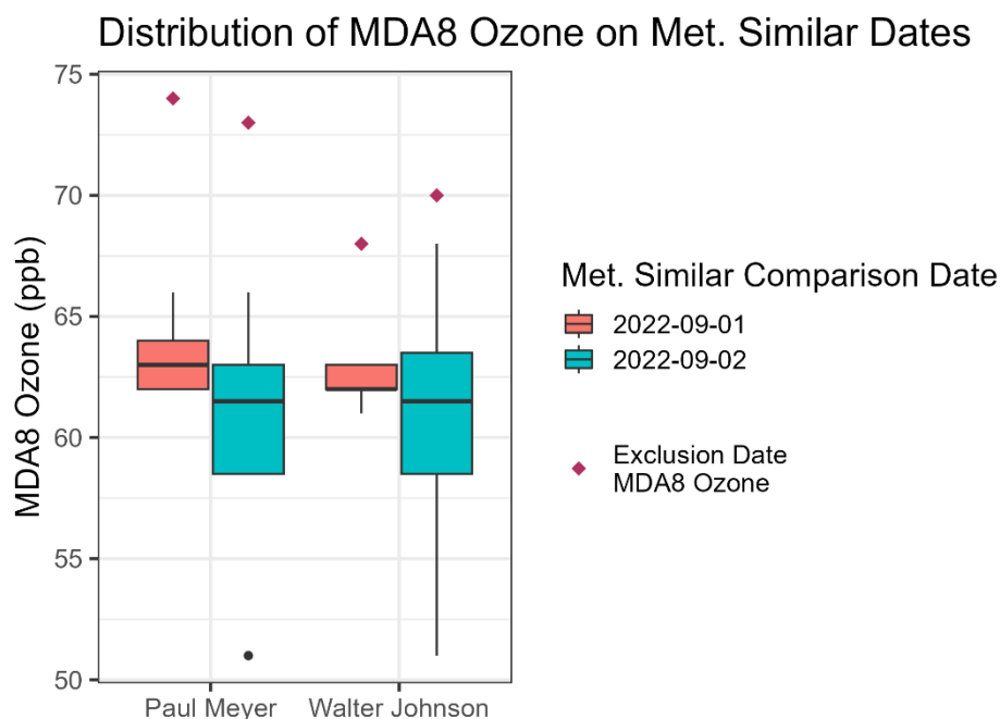
Figure 200. Distribution of MDA8 ozone concentrations on meteorologically similar days at the Paul Meyer and Walter Johnson measurement sites during the exclusion period, September 1, 2022 (pink boxes) and September 2, 2022 (green boxes). MDA8 ozone concentrations measured per site on each exclusion date are plotted as red diamonds.
