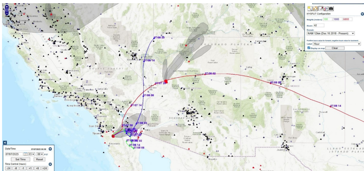
Figure 232. 42-hr forward trajectory from the NAM model arriving in southeast Clark County on July 8, 2023, at 14:00 PST at 1,000 m (blue line) AGL, 100 m (green line) and 6,000 m (red line) AGL, HMS fires (triangles), and smoke (gray shading) on are also displayed. Image courtesy of EPA's AirNow-Tech.
