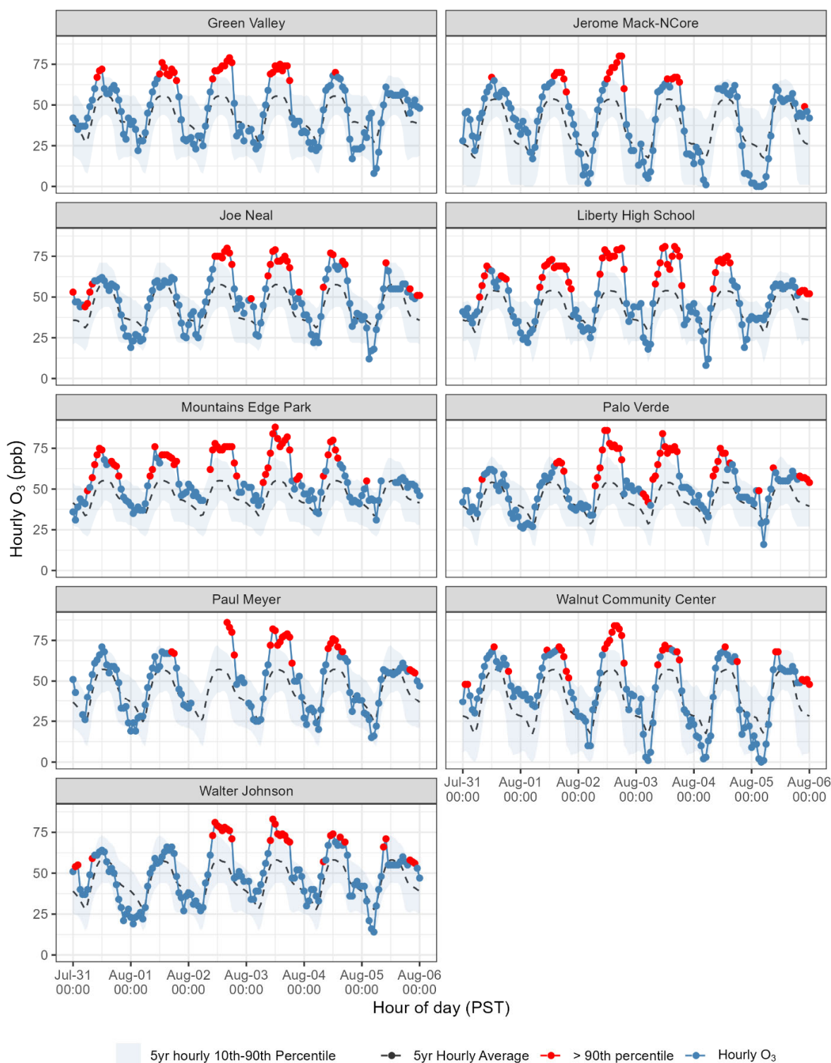
Figure 79. Hourly ozone concentrations (ppb) compared to 5-yr* ozone season (May 1-October 31) hourly means and 10-90th percentiles. *Note: data from the Liberty High School, Mountain's Edge, and Walnut Community Center sites began less than five years ago.
