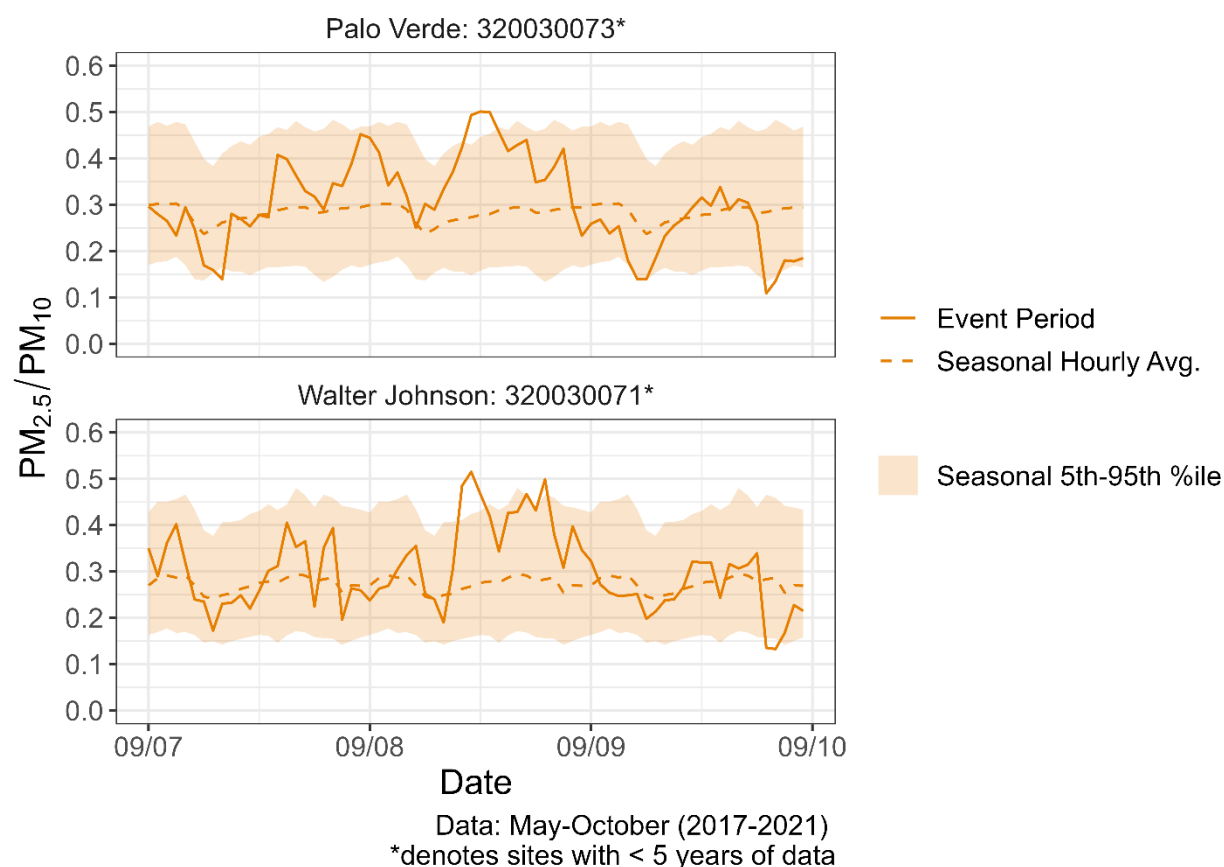
Figure 130. Ratio of PM_{2.5} -to- PM_{10} concentrations at the Palo Verde (top) and Walter Johnson (bottom) sites before and during the September 9 event period. The 5-yr average PM_{2.5} -to- PM_{10} diurnal ratio is displayed as a dotted line, and the 5th-95th percentile range is shown as a shaded ribbon. The 5th-95th percentile concentration is calculated across the ozone production season (May-October) of 2017-2021.
