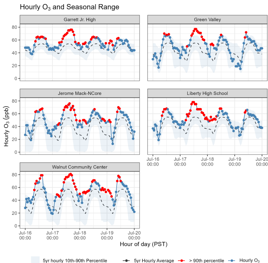
Figure 146. Hourly ozone concentrations (ppb) compared to 5-yr ozone season (May 1–October 31) hourly means and 10th–90th percentiles. Data collection did not begin until 2021 at Garrett Jr. High, Liberty High School, and Walnut Community Center, so data for these sites begins from the first available date in 2021.
