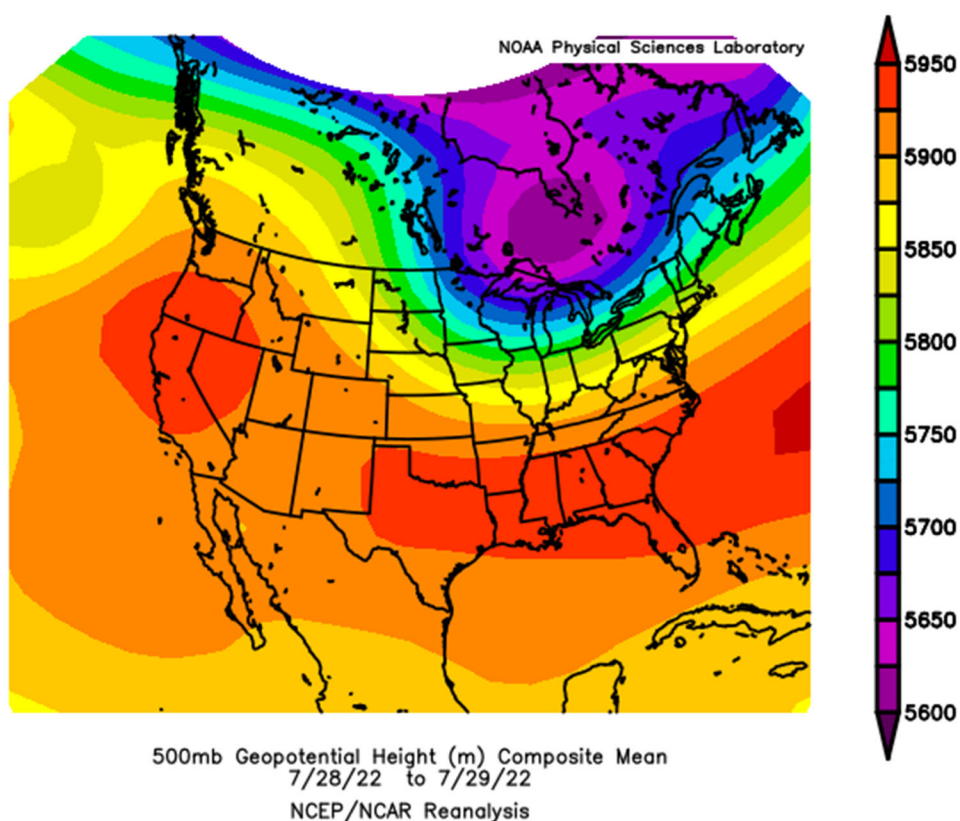
Figure 168. Mean 500 mb geopotential heights (m) for the July 28-29, 2022, period. The dark orange shading over California, Oregon, and Nevada denotes a high-pressure system. Source: NOAA
