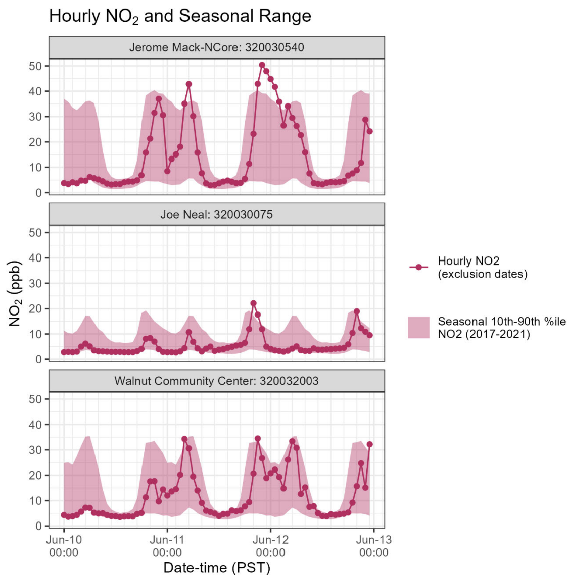
Figure 52. Hourly NO 2 measurements overlaid on the 10th-90th percentile diurnal concentration at all affected sites.
