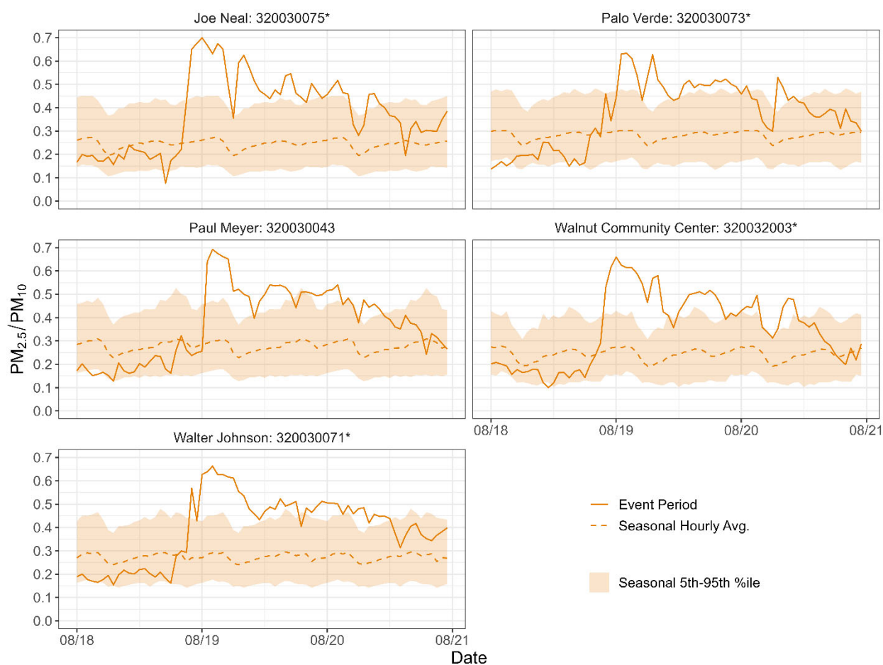
Figure 115. Ratio of PM_{2.5} -to- PM_{10} concentrations at the affected sites during the August 19 event period. The 5-yr average PM_{2.5} -to- PM_{10} diurnal ratio is displayed as a dotted line, and the 5th-95th percentile range is shown as a shaded ribbon. The 5th-95th percentile concentration is calculated across the ozone production season (May-October) of 2017-2021.
