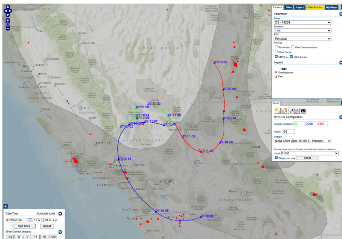
Figure 285. 36-hr boundary-layer backward trajectories from the NAM model ending at 13:00 PST on July 11, 2024, at 50 m (green line), 3,000 m (blue line), and 6,350 m (red line). HMS fires (triangles) and smoke (gray shading) on July 10 are also displayed. Image courtesy of EPA's AirNow-Tech.
