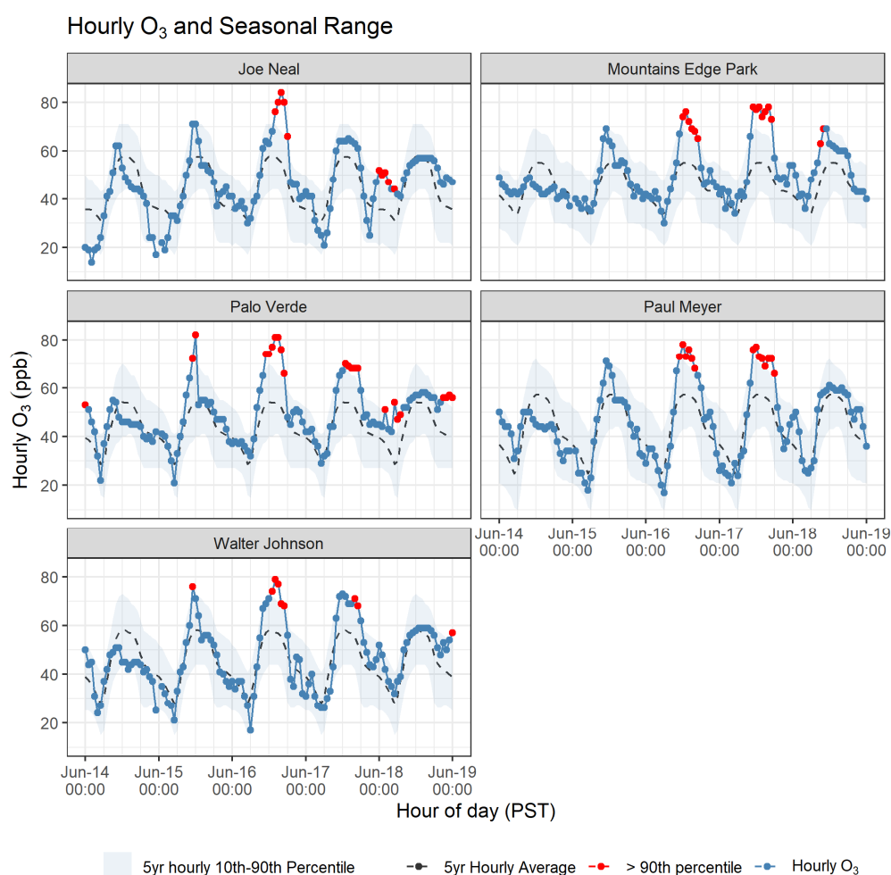
Figure 54. Hourly ozone concentrations (ppb) compared to 5-yr* ozone season (May 1-October 31, 2017-2021) hourly means and 10-90th percentiles. *Note: data from the Mountain's Edge site are only available for June 1-October 31, 2021.
