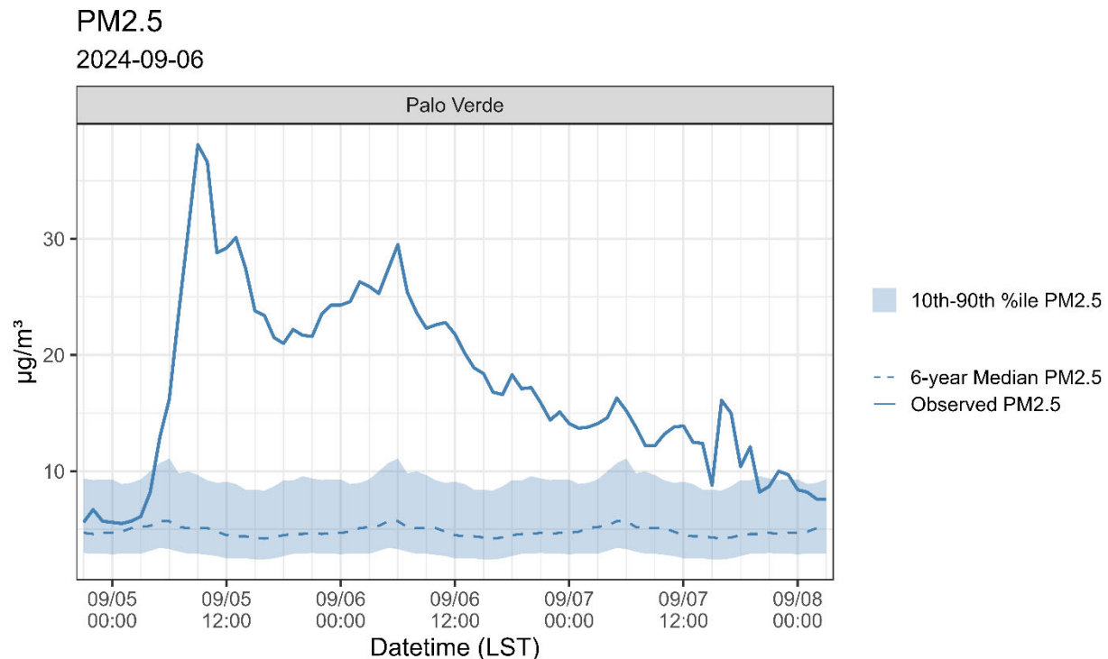
Figure 348. Hourly PM_{2.5} measurements from September 5-8, 2024, overlaid on the 10th-to-90th percentile diurnal concentrations at the Palo Verde site (AQS site code 320030073). The 10th-to-90th percentile concentration is calculated across the ozone production season (April-September) of 2019-2024.
