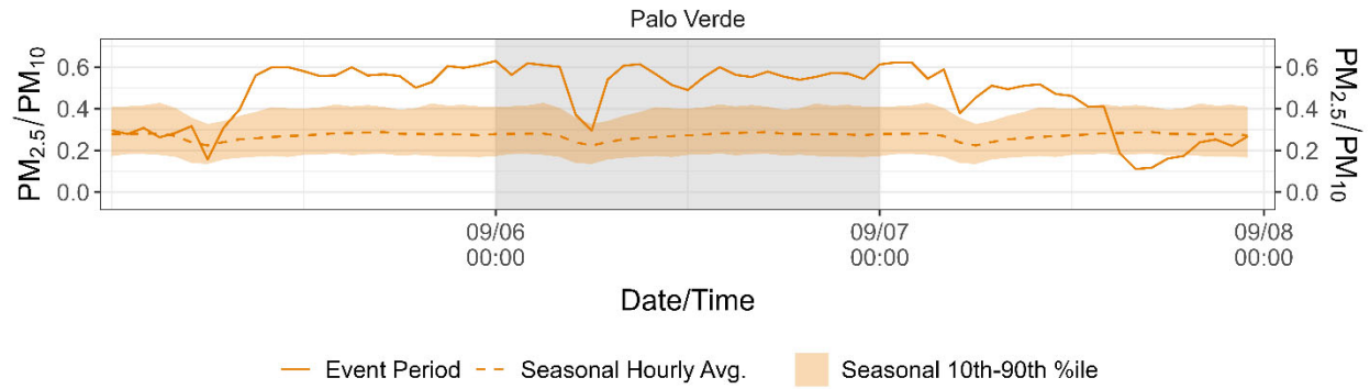
Figure 349. Ratio of PM_{2.5} -to- PM_{10} concentrations during the event period overlaid on the 10th-to-90th percentile diurnal concentrations at the Palo Verde site (AQS site code 320030073). The 10th-to-90th percentile concentration is calculated across the ozone production season (April-September) of 2019-2024. The date of September 6, 2024, is shaded in grey.
