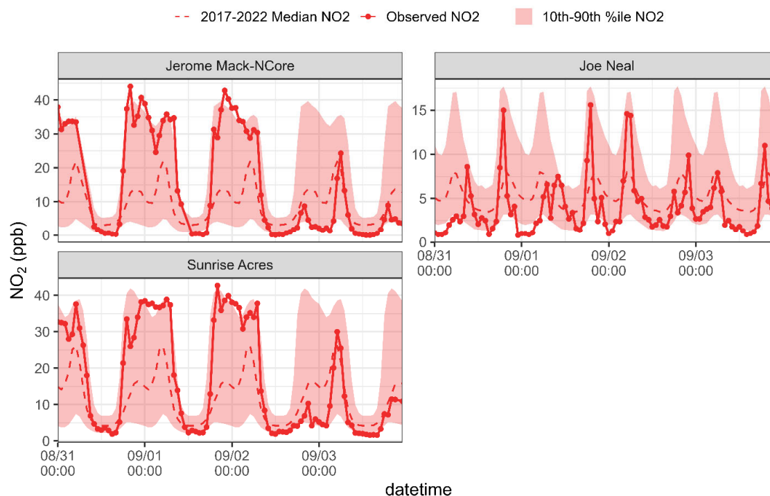
Figure 198. Hourly NO 2 measurements overlaid on the 10th-90th percentile diurnal concentrations at each event-affected measurement site and supporting sites that measure NO 2 concentrations. The 10th-90th percentile concentration is calculated across the ozone production season (May-October) of 2017-2022.
