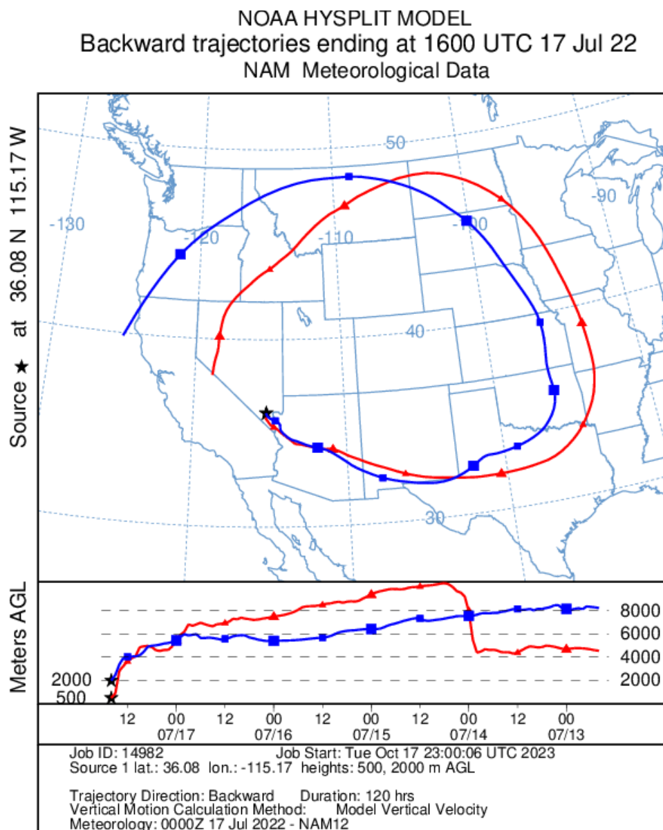
Figure 153. HYSPLIT back trajectory initiated at 16:00 UTC (08:00 PST) on July 17, 2022, using NAM 12 km meteorology. The back trajectory ran for 120 hours, ending in Las Vegas (36.08, -115.17) at 500 m and 2,000 m AGL.
