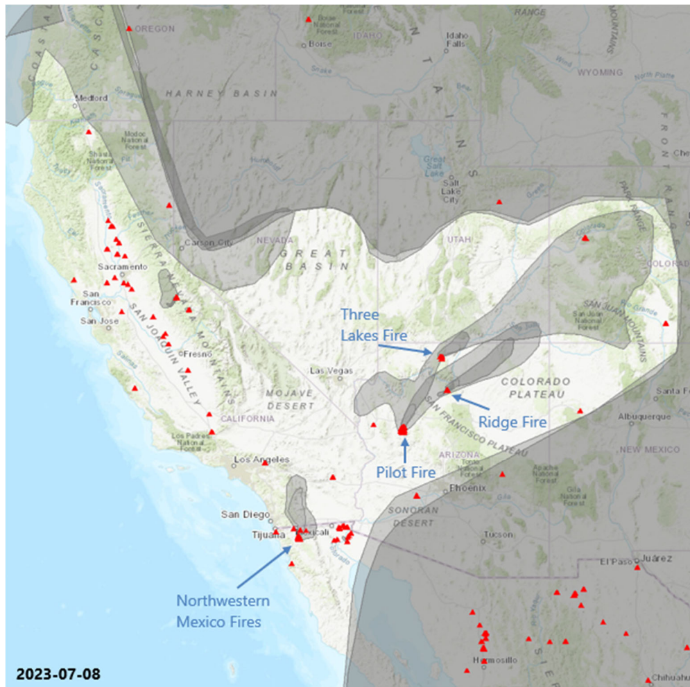
Figure 217. NOAA HMS smoke analysis (grey contours) and satellite fire detections (red triangles) for July 8, 2023. Source: AirNow-Tech.
