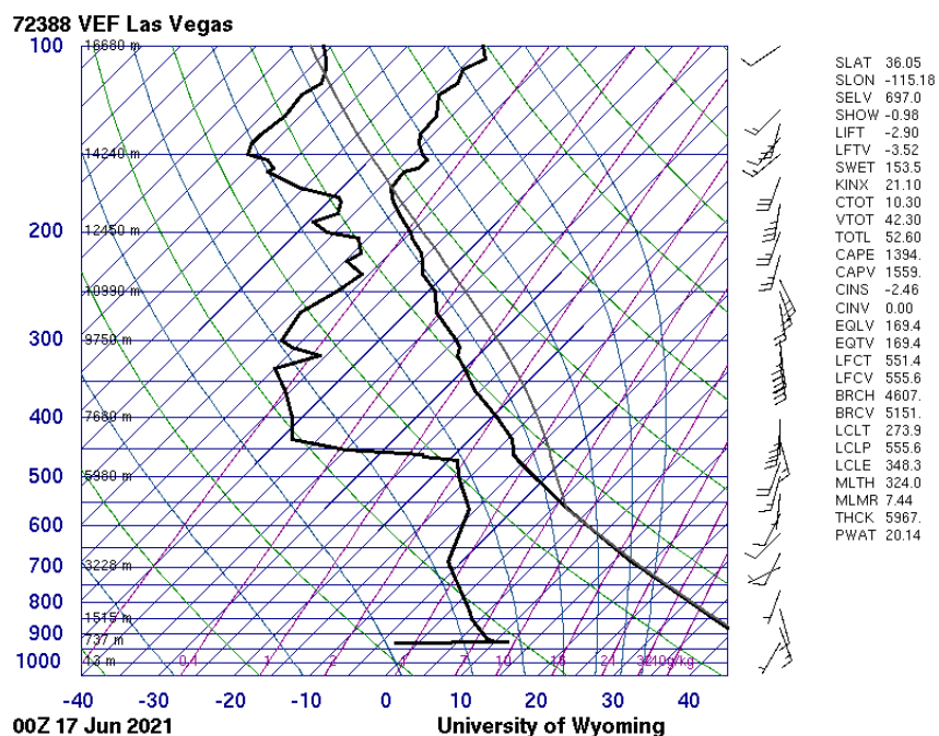
Figure 59. Sounding from Las Vegas, Nevada, at 00:00 UTC on June 17 (16:00 PST on June 16), 2021, where x-axis shows temperature (°C) and y-axis shows pressure (mb). Retrieved from https://weather.uwyo.edu/upperair/sounding.html .
