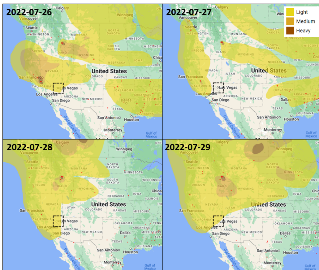
Figure 164. HMS smoke maps for July 26-29, 2022, showing smoke transport and qualitative smoke density. Clark County, NV, is enclosed by a dashed, black box on each map.
