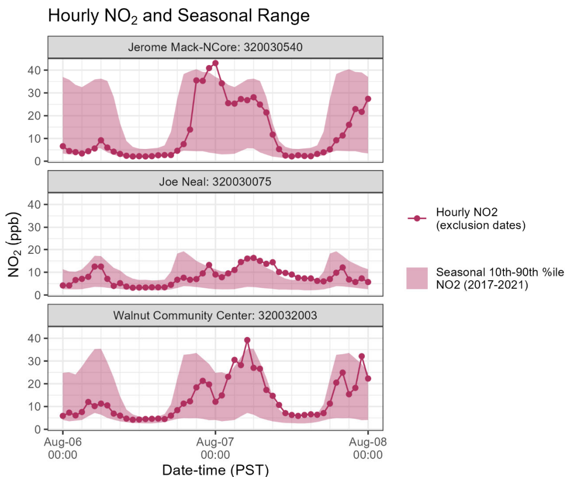
Figure 100. Hourly NO 2 measurements overlaid on the 10th-90th percentile diurnal concentration at affected sites that measure NO 2 . The 10th-90th percentile concentration is calculated across the ozone production season (May-October) of 2017-2021.
