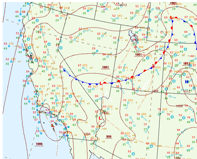
Figure 255. Surface weather conditions at 07:00 PST on June 16, 2024. Image courtesy of NOAA's Weather Prediction Center.
