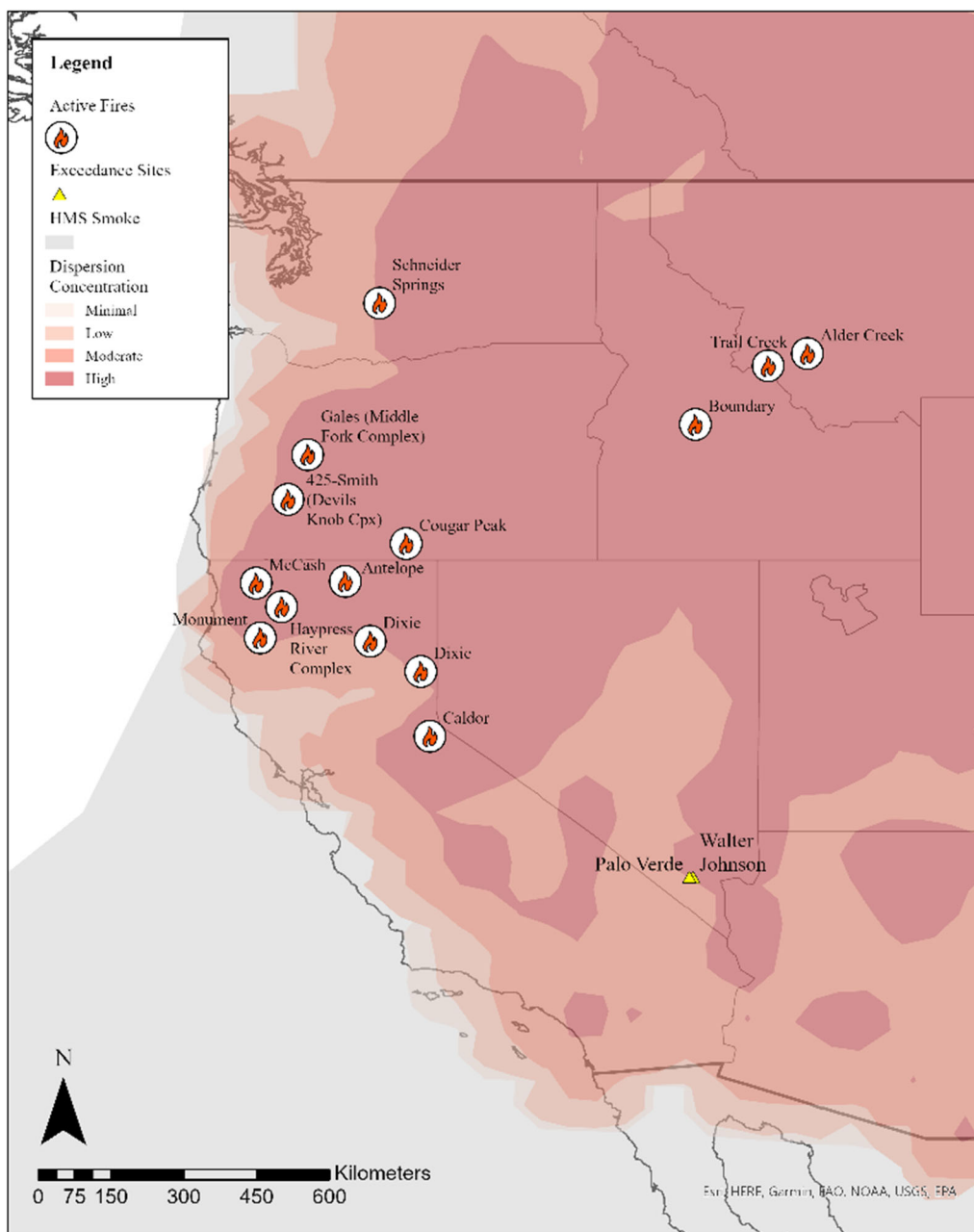
Figure 121. HYSPLIT dispersion modeling for 13 large fires (labeled as “Active Fires”) throughout the western U.S. GDAS 1.0° meteorological data was used, and dispersion was initiated on September 5 at 06:00 PST to model the regional smoke observed in satellite and HMS products. HMS smoke is shown in gray and qualitative concentrations of particulate matter are shown in shades of red. Accumulation of particulate matter is shown at 0–100 m for 06:00 PST on September 8 through 06:00 PST on September 9, 2021. Note: the Dixie Fire is labeled twice because there was a significant distance between the active burning edges of the fire on these dates.
