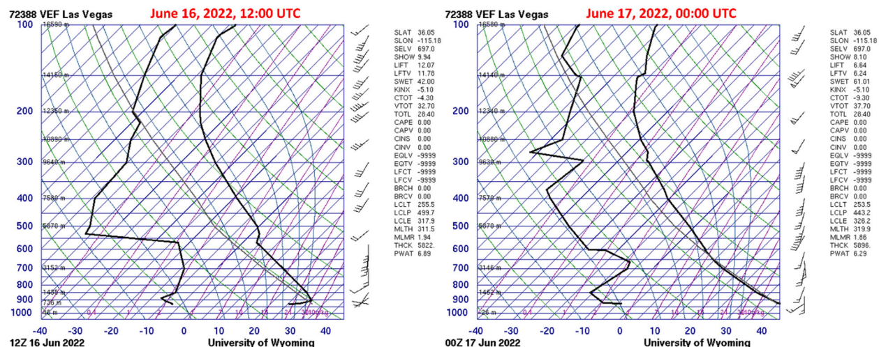
Figure 135. Skew-T soundings launched from KVEF on June 16, 2022, at 12:00 UTC (04:00 PST) (left), and June 17 at 00:00 UTC (June 16 at 16:00 PST) (right).
