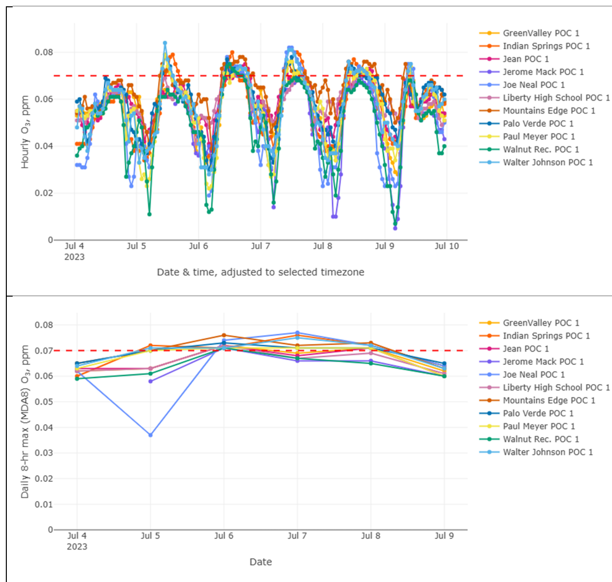
Figure 201. Top: Hourly ozone concentrations (ppm) across July 4-10, 2023. Bottom: Daily 8-hour maximums (ppm) that exceeded the NAAQS across July 4-10, 2023.
