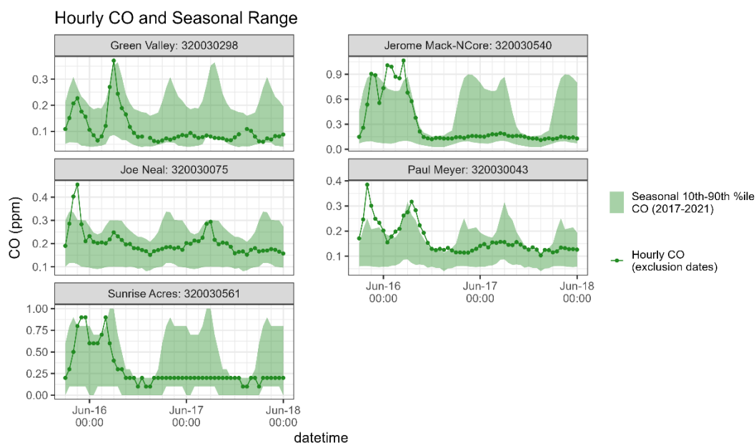
Figure 142. Hourly CO measurements overlaid on the 10th-90th percentile diurnal concentration at the event-affected sites and supporting sites that measure CO. The 10th-90th percentile concentration is calculated across the ozone production season (May-October) of 2017-2022.
