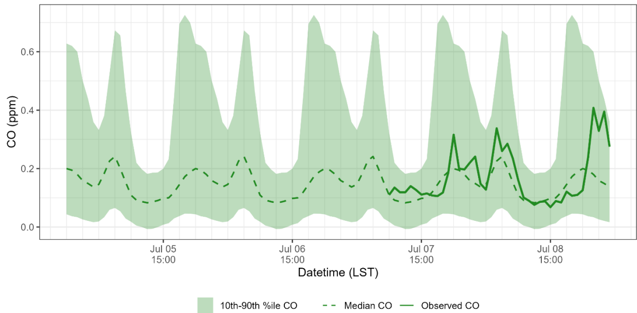
CO - Walnut Rec (320032003) 2023-07-05 to 2023-07-08
