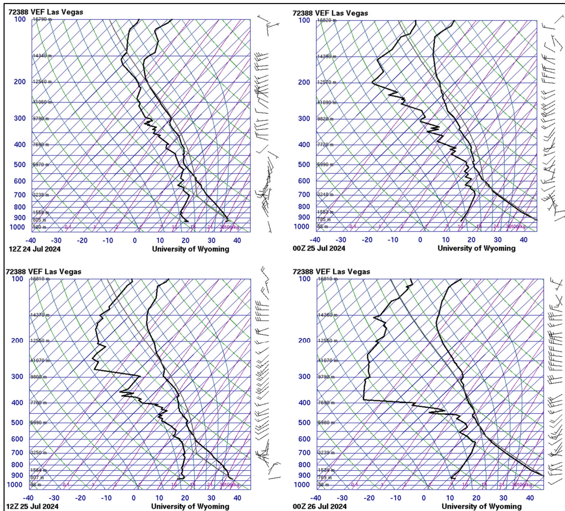
Figure 330. Observed soundings from 04:00 PST (left panels) and 16:00 PST (right panels) from July 24, 2024 (top) and July 25, 2024 (bottom). Source: University of Wyoming.
