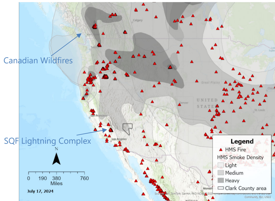
Figure 299. Continental view of HMS fire detections (red triangles) and smoke density (grey contours) on July 17, 2024. Clark County is outlined in grey.
