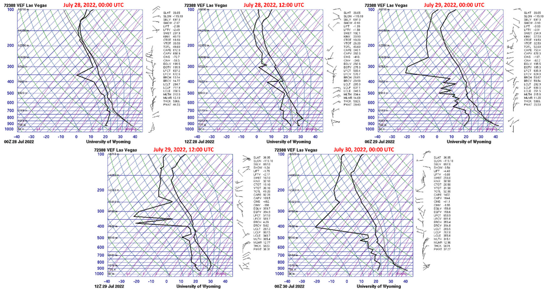
Figure 167. Skew-T soundings launched from KVEF from July 28, 2022, at 00:00 UTC (July 27 at 16:00 PST) (top left), to July 30 at 00:00 UTC (July 29 at 16:00 PST) (bottom right).
