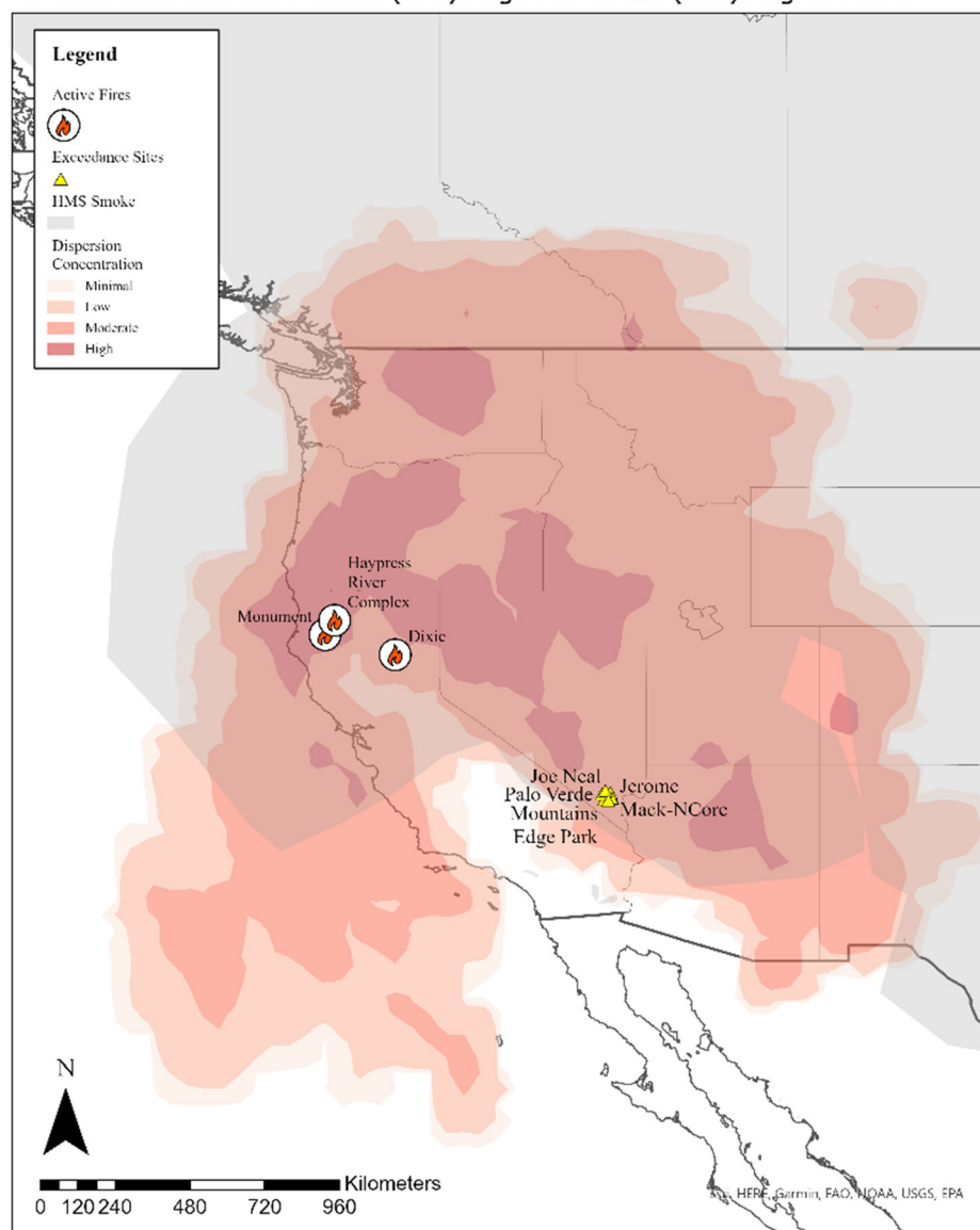
Figure 82. Results of the HYSPLIT dispersion modeling for three large fires (labeled as “Active Fires”) in California. GDAS 1.0° meteorological data was used, and dispersion was initiated on August 1, 2021, at 00:00 PST to model the regional smoke observed in satellite and HMS products. HMS smoke is shown in gray and qualitative concentrations of particulate matter are shown in shades of red. Accumulation of particulate matter is shown at 0-100 m for 00:00 PST on August 2 through 00:00 PST on August 4, 2021.
