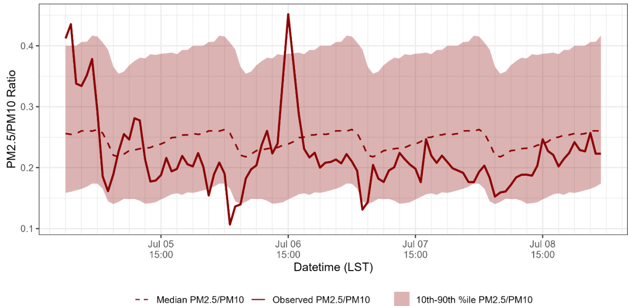
PM2.5/PM10 - Palo Verde (320030073) 2023-07-05 to 2023-07-08
