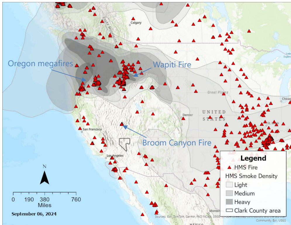
Figure 338. Continental view of HMS fire detections (red triangles) and smoke density (grey contours) from September 6, 2024. Clark County is outlined in grey.
