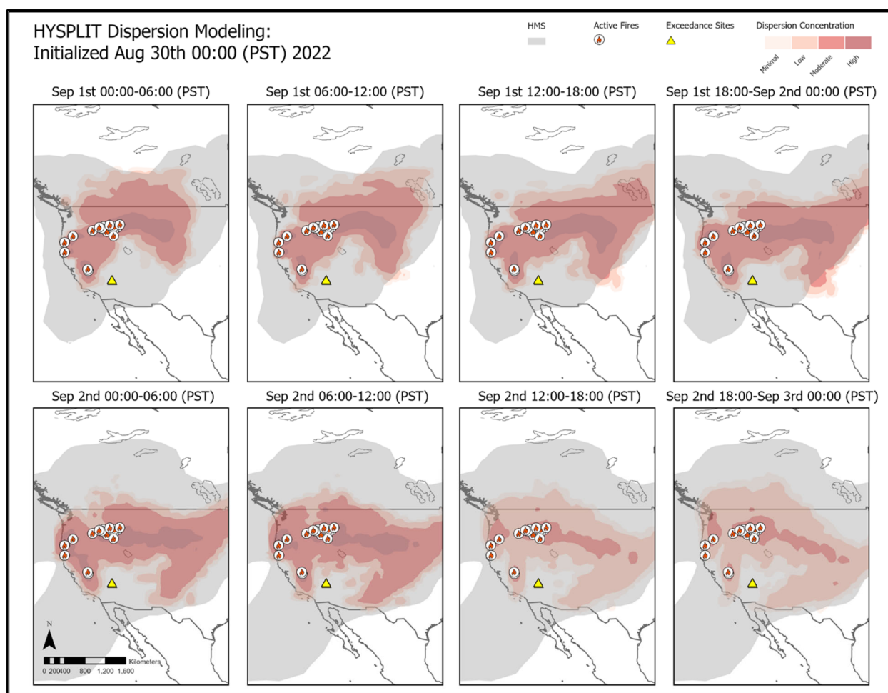
Figure 191. HYSPLIT dispersion modeling for 17 large fires (labeled as “Active Fires”) in the western U.S. on or before the exclusion dates of September 1-2, 2022. GDAS 1.0° meteorological data was used, and dispersion was initiated on August 30, at 00:00 PST, to model the regional smoke observed in satellite and HMS products. HMS smoke is shown in gray, and qualitative concentrations of particulate matter are shown in shades of red. Accumulation of particulate matter is shown at 0-4,500 m.
