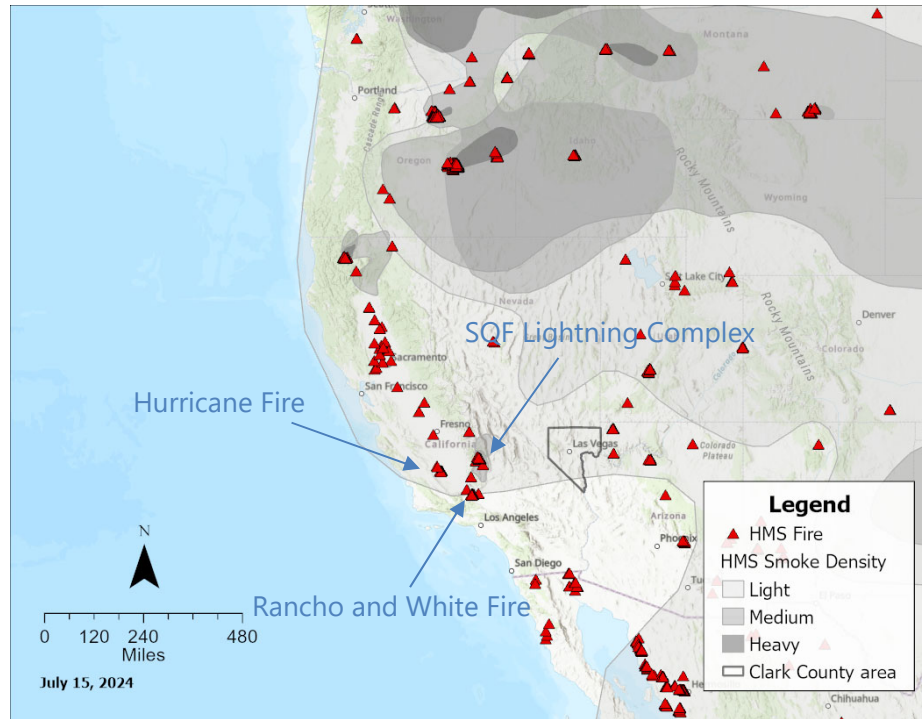
Figure 297. View of the western United States with HMS fire detections (red triangles) and smoke density (grey contours) on July 15, 2024. Clark County is outlined in grey.
