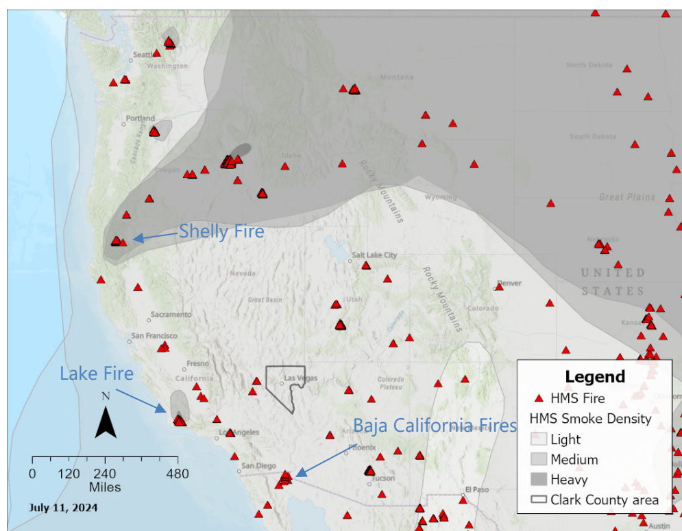
Figure 268. Western U.S. view of HMS fire detections and smoke density on July 11, 2024.
