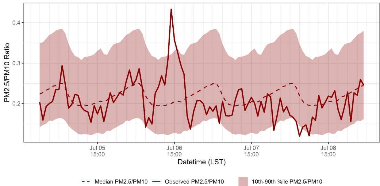
PM2.5/PM10 - Mountains Edge (320030044) 2023-07-05 to 2023-07-08
