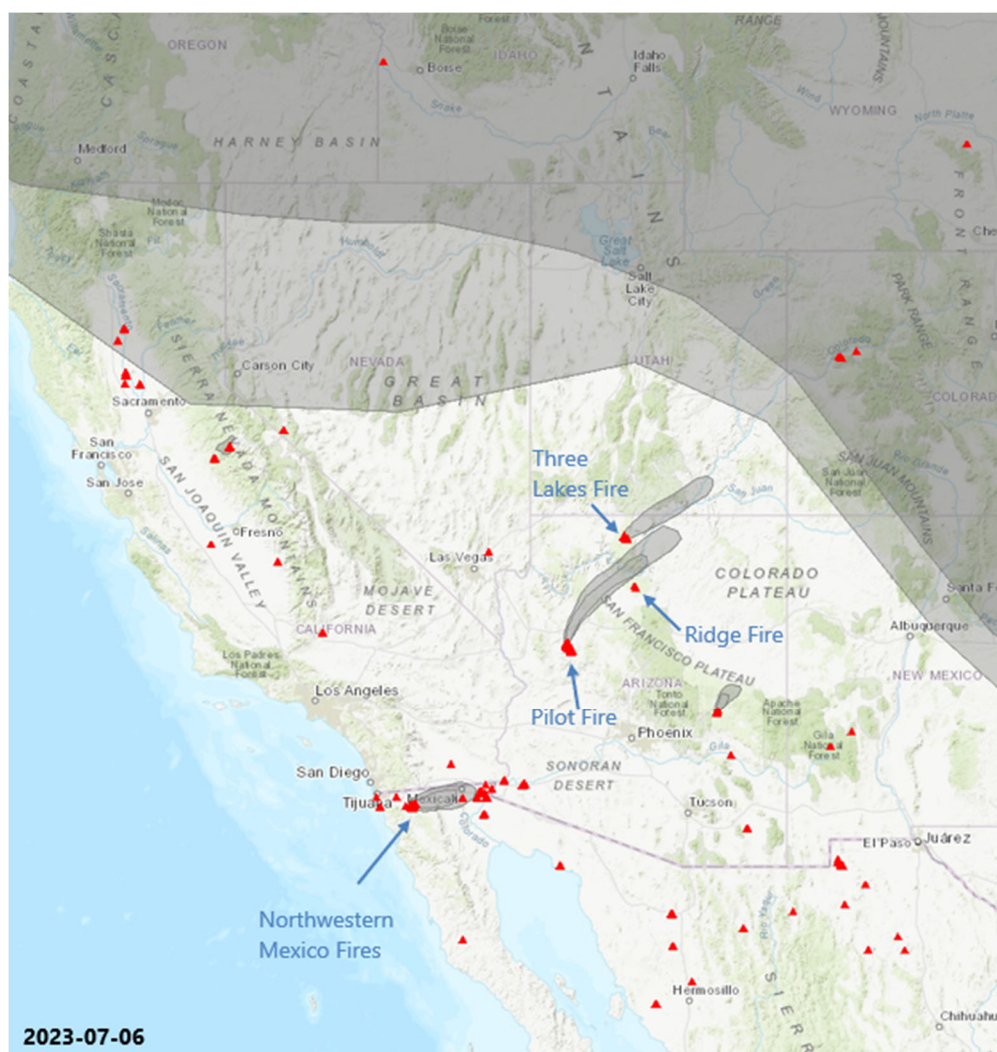
Figure 215. NOAA HMS smoke analysis (grey contours) and satellite fire detections (red triangles) for July 6, 2023. Source: AirNow-Tech.
