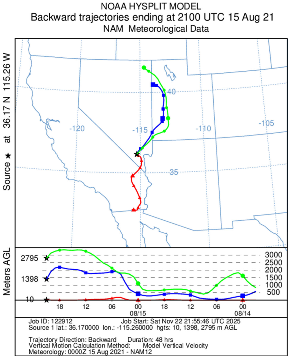
Figure C-7. Back-trajectories initiated on August 15, 2021, at 21:00 UTC (13:00 PST).
