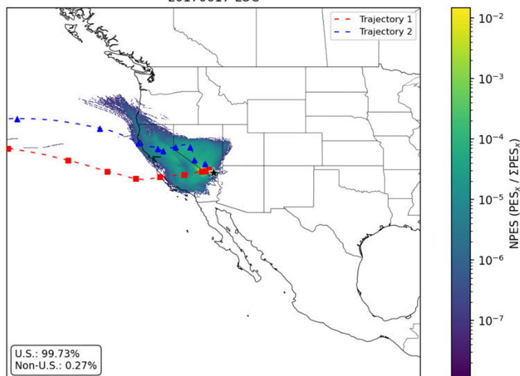
Clark County 179B Demo: HYSPLIT 5d Back Dispersion Dataset [NPES, 0-5km] 20170617-LOC
