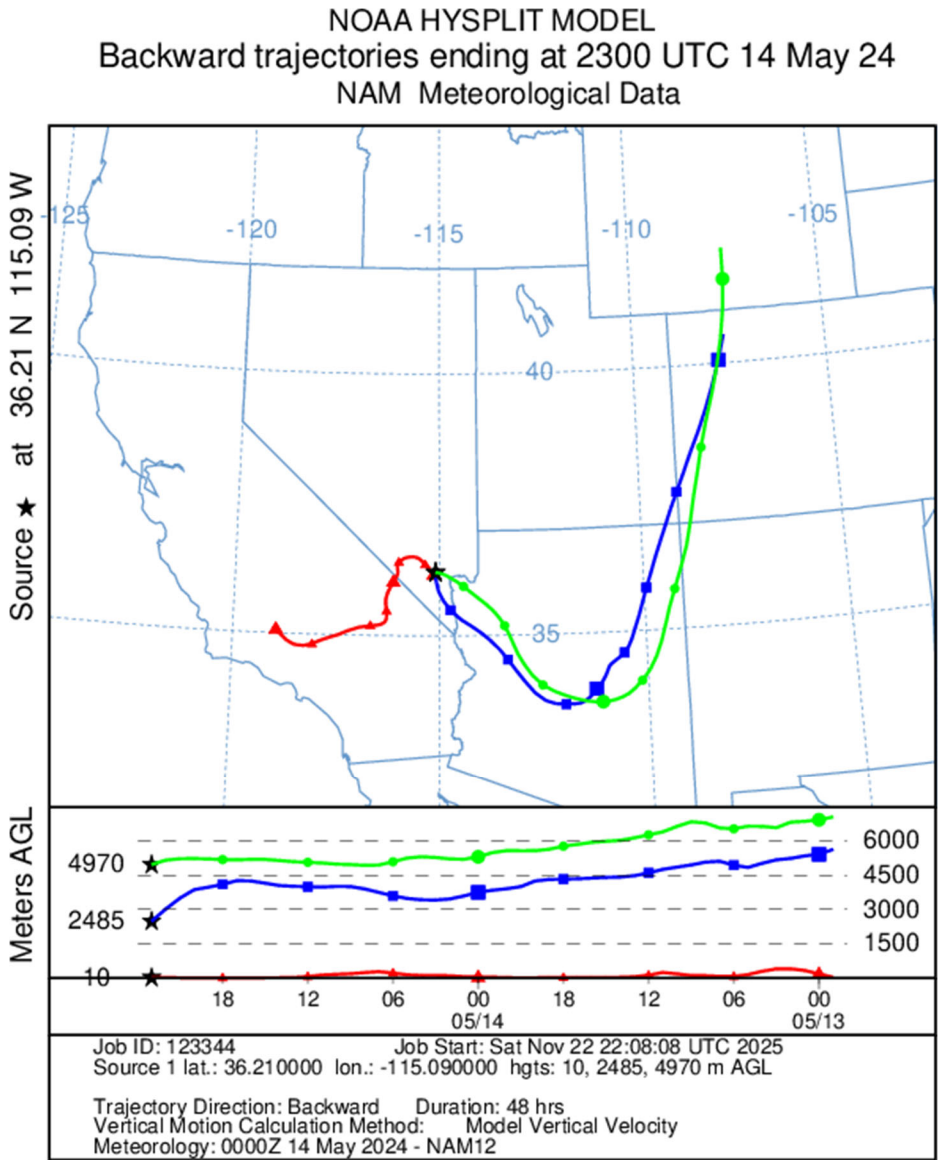
Figure C-10. Back-trajectories initiated on May 14, 2024, at 23:00 UTC (15:00 PST).
