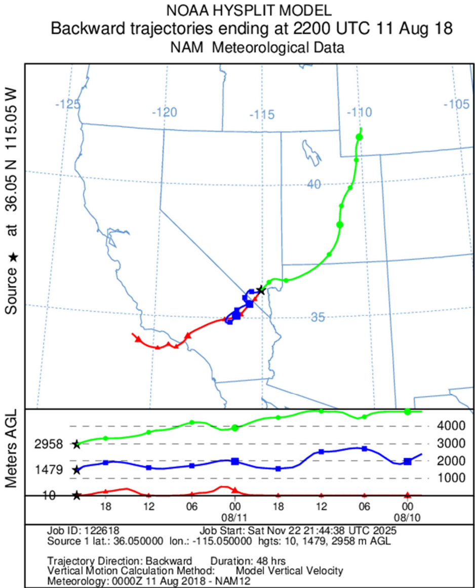
Figure C-4. Back-trajectories initiated on August 11, 2018, at 22:00 UTC (14:00 PST).
