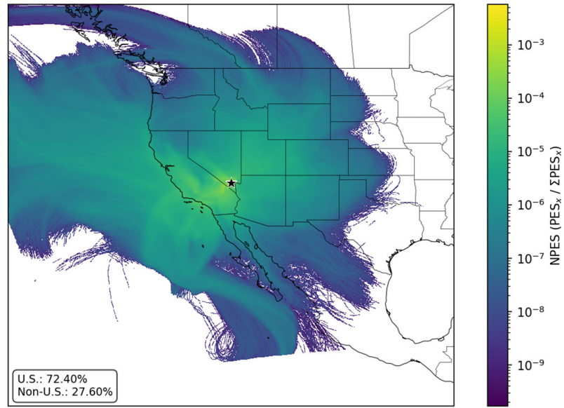
Figure 10. Clark County 5-day back dispersion-based NPES; the results are compiled for the 10 selected exceedance days (see Table 6 ) with the local transport (LOC) air transport regime. NPES is based on the average concentration of a generic, inert tracer gas between 0 and 5 km.
