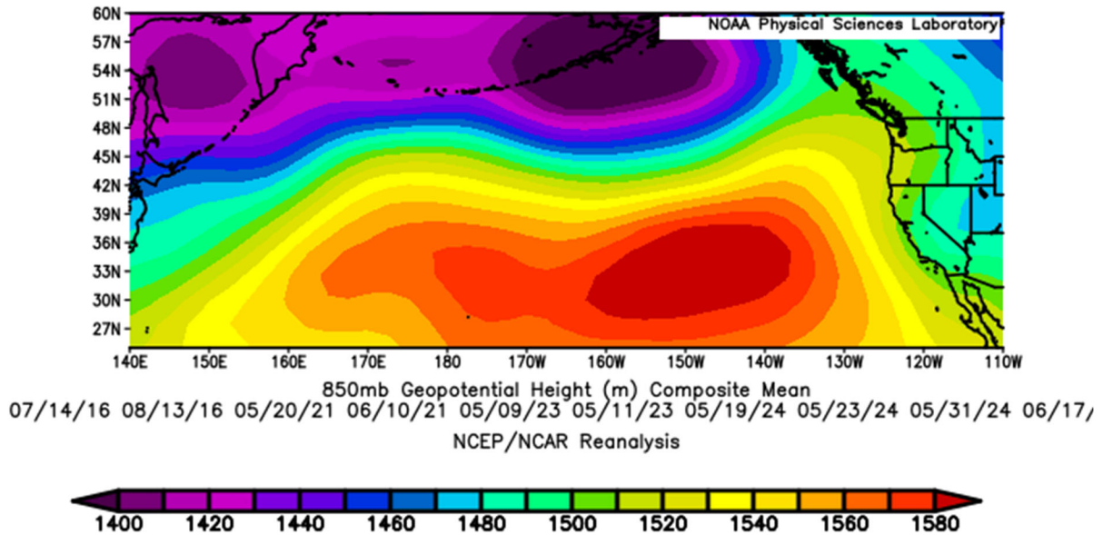
Figure 29. Mean geopotential height at 850 mb on LNR transport days. Source: NOAA.
