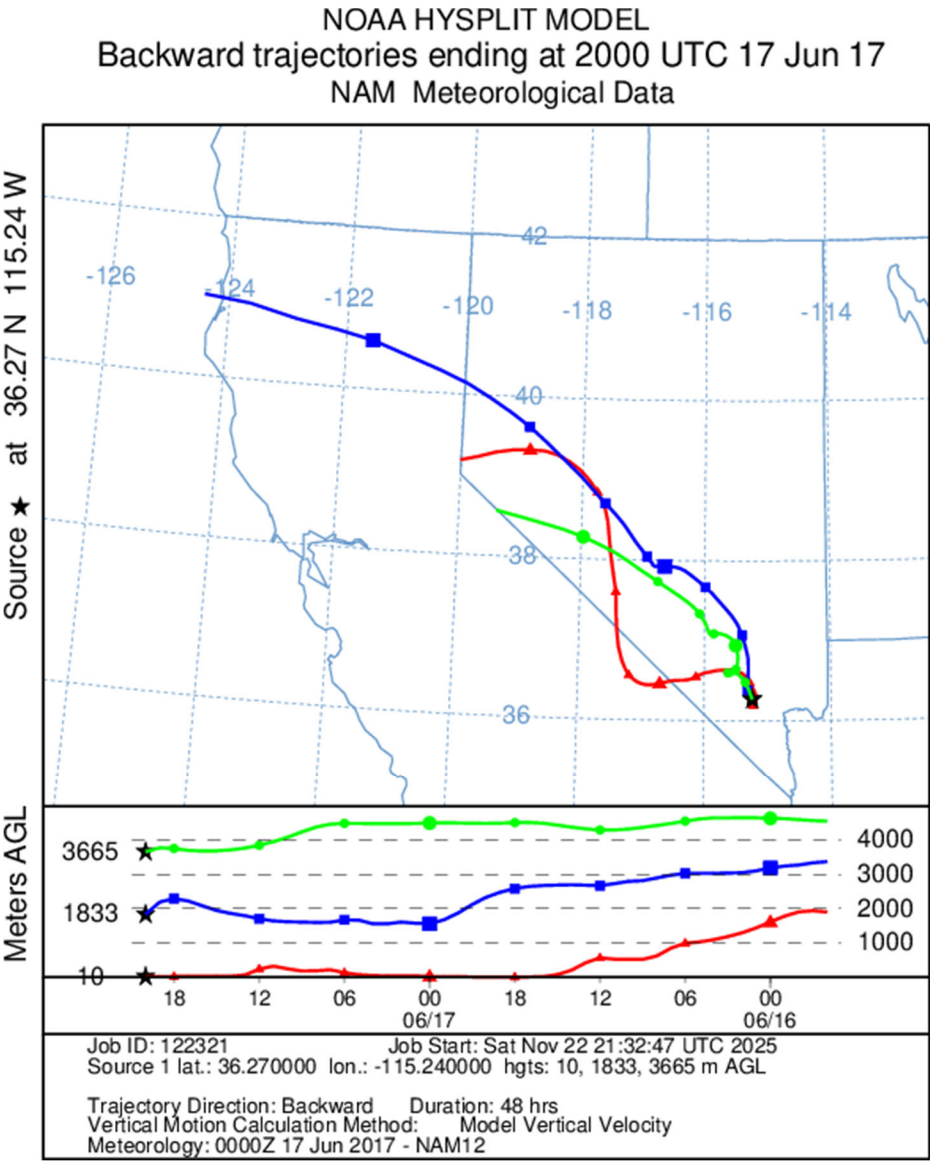
Figure C-1. Back-trajectories initiated on June 17, 2017, at 20:00 UTC (12:00 PST).
