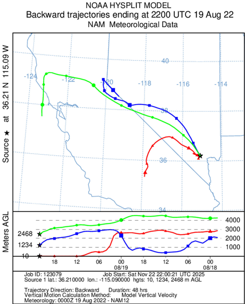
Figure C-8. Back-trajectories initiated on August 19, 2022, at 22:00 UTC (14:00 PST).
