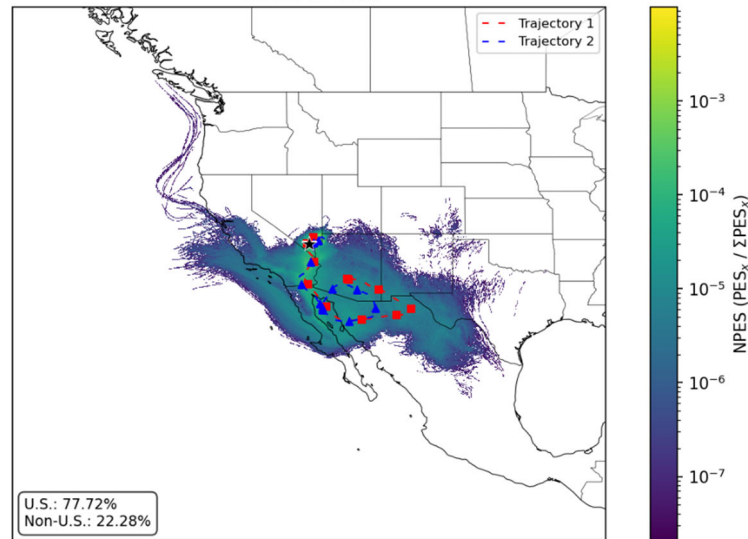
Clark County 179B Demo: HYSPLIT 5d Back Dispersion Dataset [NPES, 0-5km] 20240720-MEX
