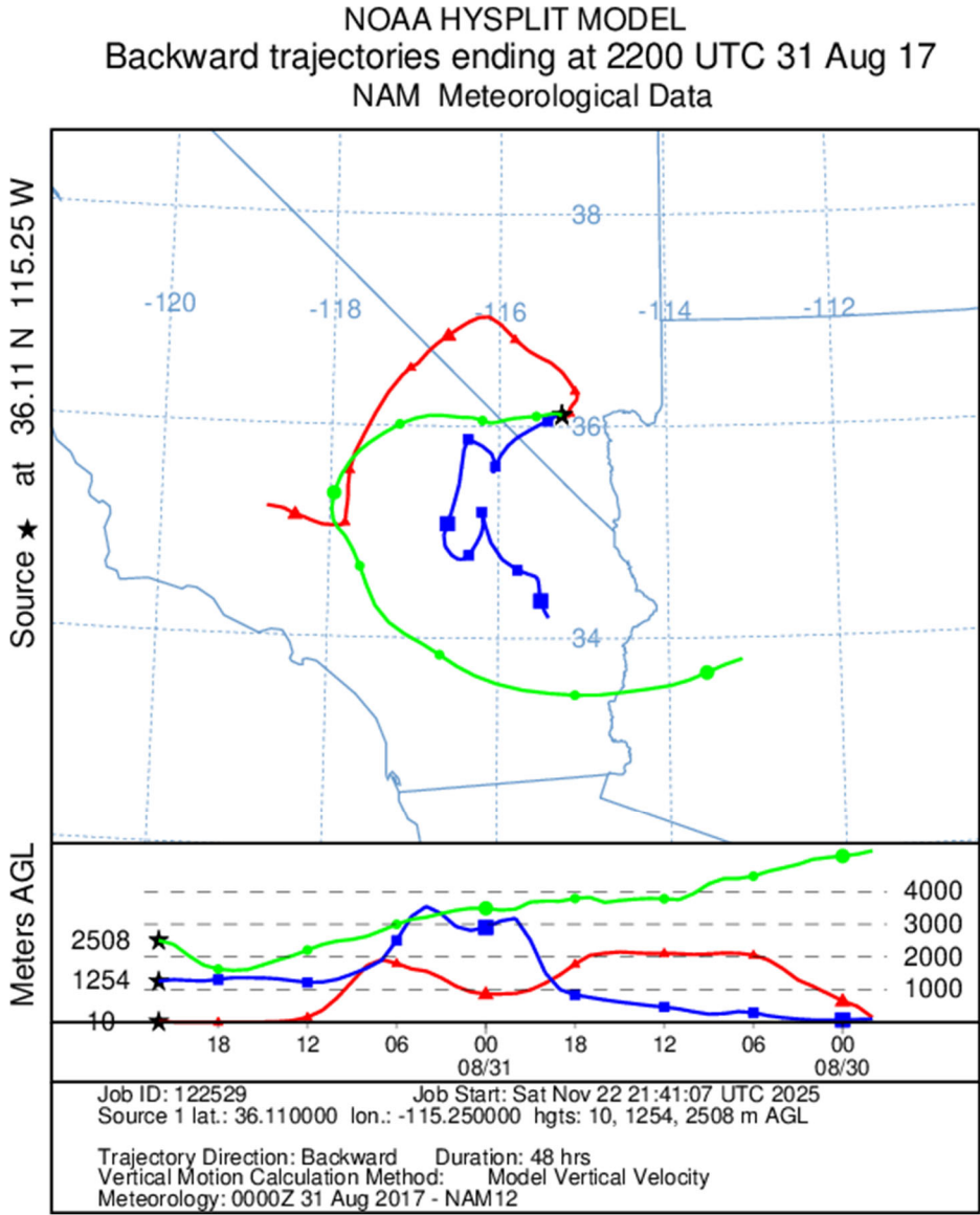
Figure C-3. Back-trajectories initiated on August 31, 2017, at 22:00 UTC (14:00 PST).
