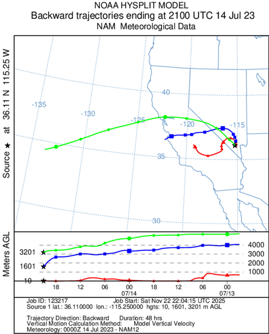
Figure C-9. Back-trajectories initiated on July 14, 2023, at 21:00 UTC (13:00 PST).
