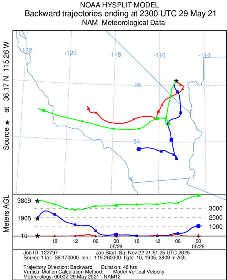
Figure C-6. Back-trajectories initiated on May 29, 2021, at 23:00 UTC (15:00 PST).
