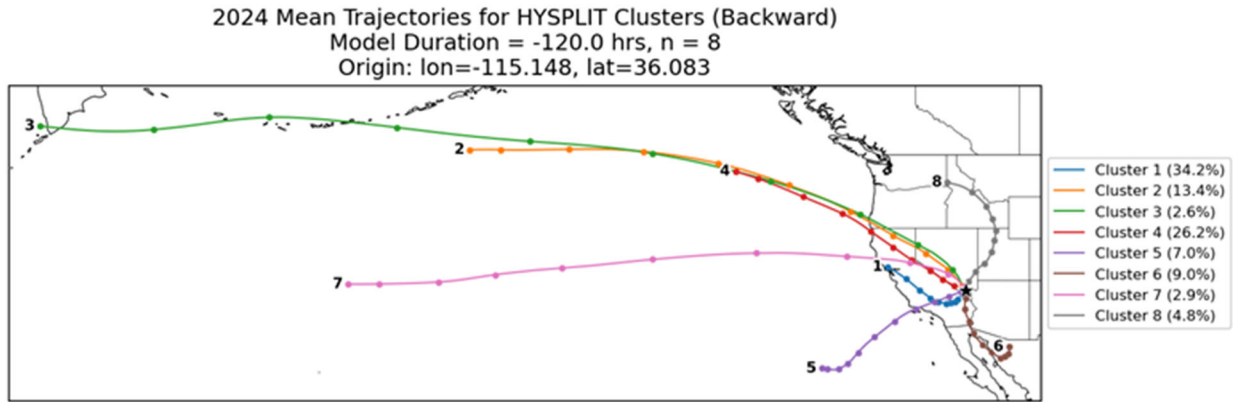
Figure A-9. Mean 5-day backward trajectories from Las Vegas, Nevada (36.0831°N, 115.1482°W), calculated using HYSPLIT cluster analysis with eight clusters for the year 2024. Each colored line represents the mean pathway of a cluster, and the percentages in the legend indicate the fraction of trajectories assigned to each cluster. Trajectories illustrate dominant transport patterns contributing to air masses arriving at the site, highlighting both regional and long-range influences on air quality.
