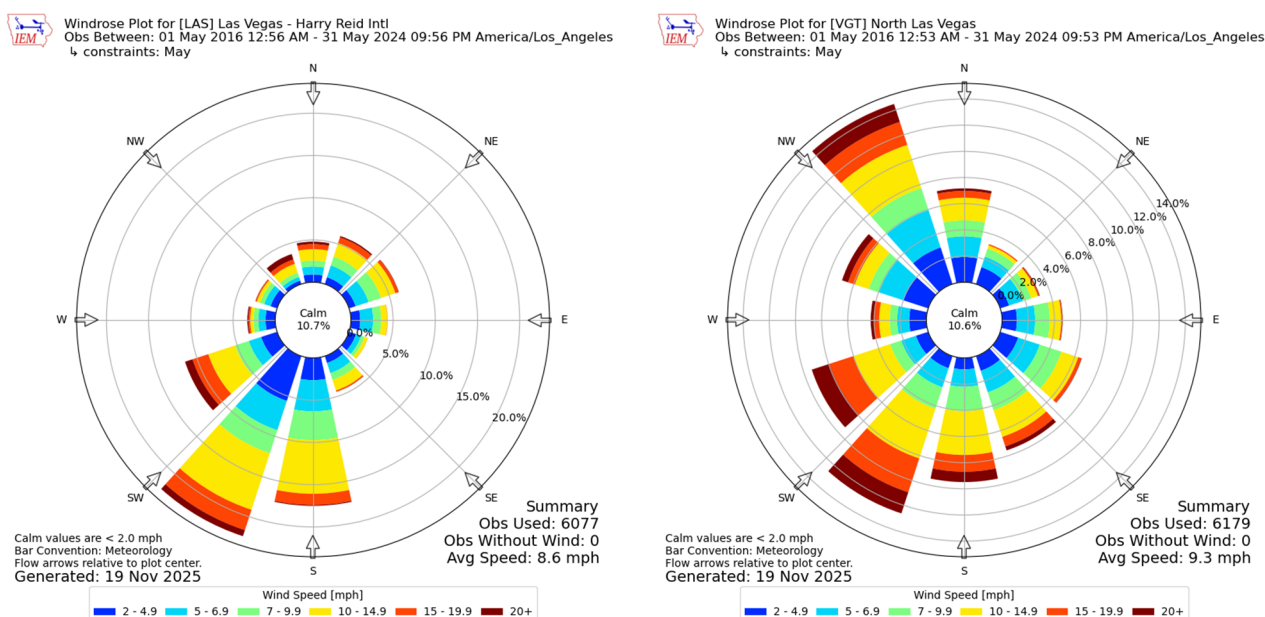
Figure 35. Wind rose diagrams for all May days from 2016-2024 at KLAS (left) and KVGT (right). Data source: Iowa State Mesonet.
